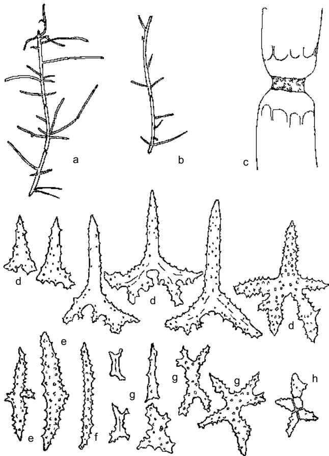
Fig 1 Primnois spicata (a) axial skeleton showing the nodes internodes and branching pattern of a branch measuring 30 mm (b) same of another branch measuring 25 mm (c) structure of a node and the surface of internode enlarged to show the surface ornamentation (d) spiny spicules different stages of growth (e) spindle - robust (f) spindle - narrow (g) multiradiate and (h) cross
