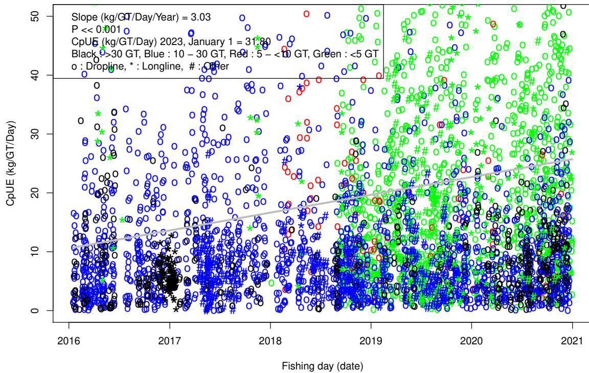
Figure 2.4: Catch per Unit of Effort in WPP 715.
