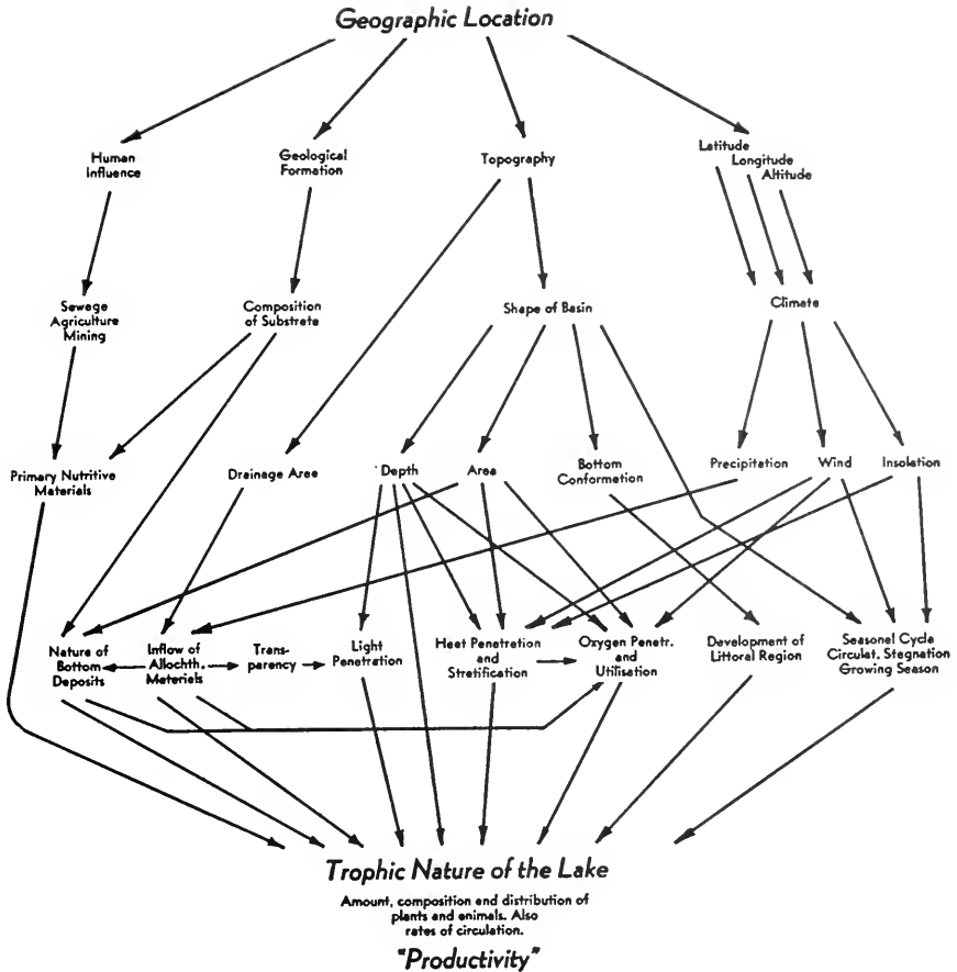
Figure 7. A diagram showing the contributions toward lake productivity by some interesting factors, both inside and outside of a body of water. After a diagram by D. S. Rawson. (By courtesy of the American Association for the Advancement of Science.)
