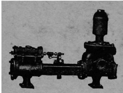
Single Vacuum Jet Condenser and General Service Steam Pumps
