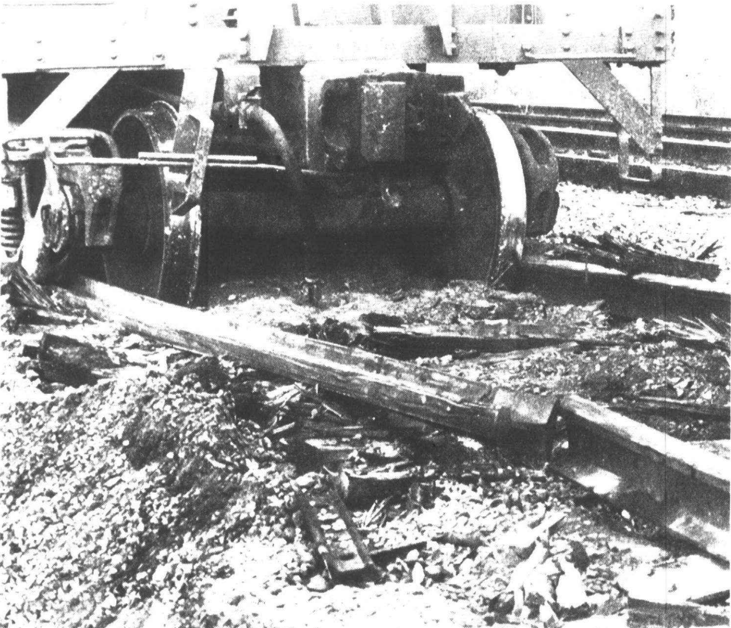
This broken section of track is believed to have caused Wednesday's derailment.
