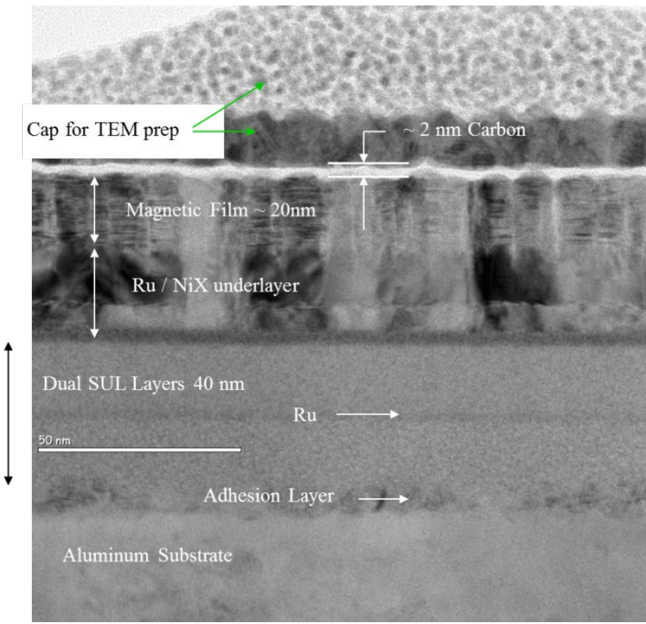
Construction of PMR media (2011) showing the complexity and the number of layers that are used. This type of construction was used for media up to around 400 Gb/in 2 areal density. (Figure 12-4)
