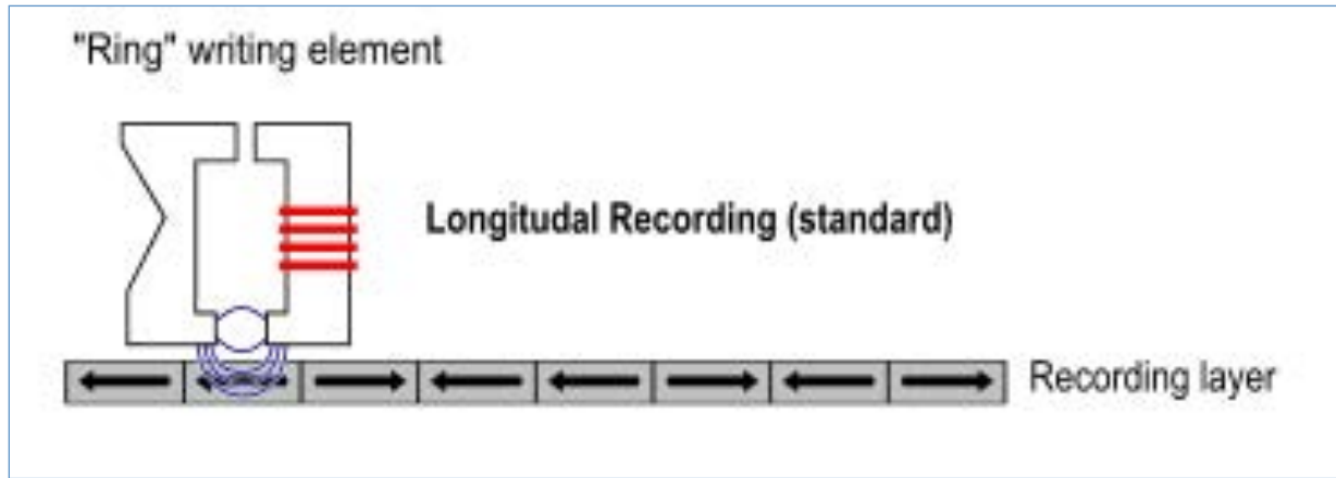
Schematic of Longitudinal Recording
