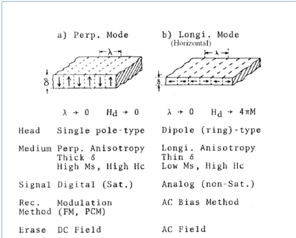
From Professor Iwasaki's 1977 paper explaining the perpendicular magnetic recording concept. (Figure 4-10)
