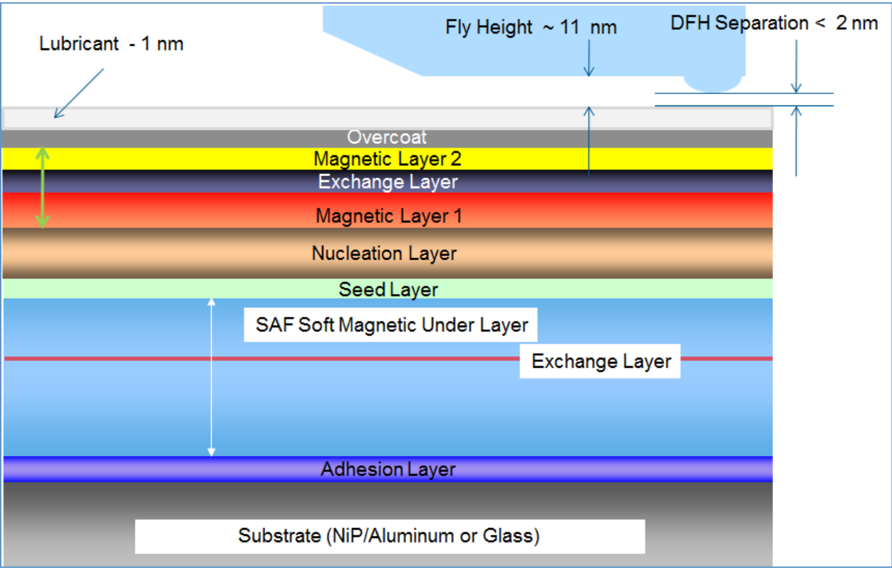
Construction of PMR media (2011) showing the complexity and the number of layers that are used. This type of construction was used for media up to around 400 Gb/in 2 areal density. (Figure 12-4)
