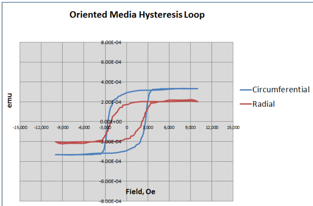
Hysteresis loop of oriented media along the texture or circumferential direction (blue) and across or radial direction to the disk (red) showing the difference in the hysteresis loop squareness .
