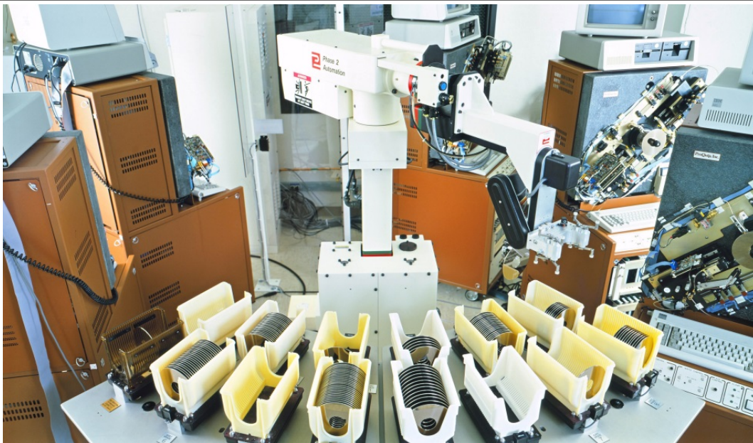
Automated disk certifier test station developed by Phase 2 Automation under the direction of Scott Chen and Steve Miura. Komag was one of the first independent media companies to develop this level of automation for disk certification. Note the IBM PC with two floppy drives which ran each ProQuip certifier.
