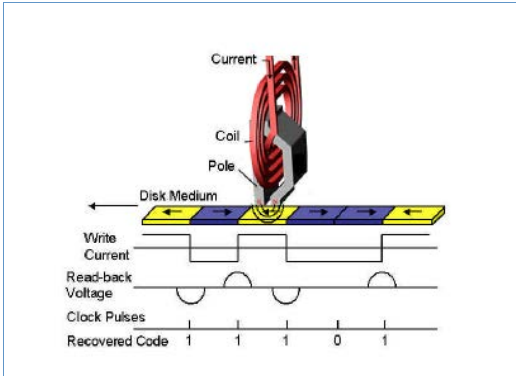
Longitudinal magnetic recording signal reproduction.
