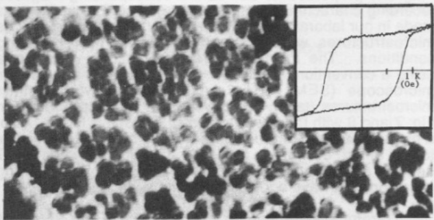
Fig. 6(c) Isolated particles, 70μ (B-H loop insert)
