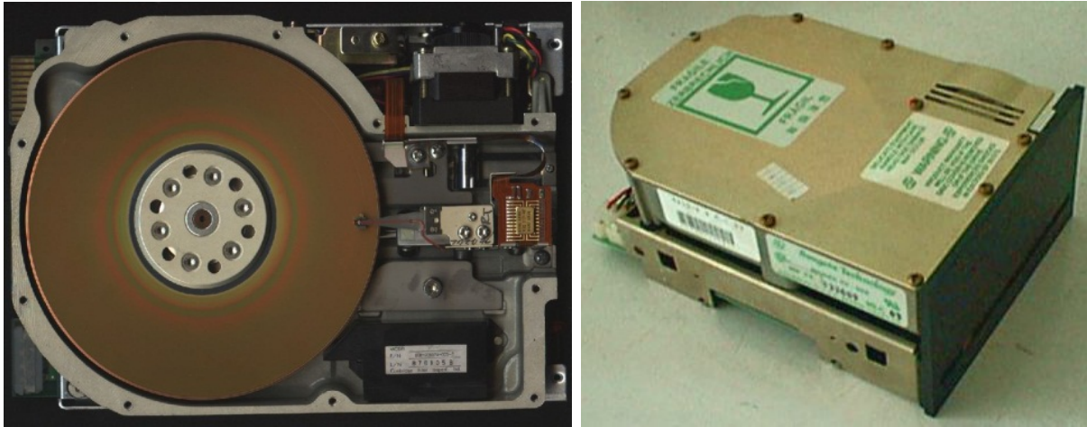
Seagate ST-506 Drive, designed to fit into 5¼-inch floppy bay of IBM PC. Drive had 5MB capacity on 2 oxide disks.
