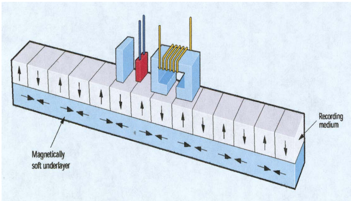
Schematic representation of a perpendicular magnetic recording arrangement (Figure 12-1). (Figure 12-1)
