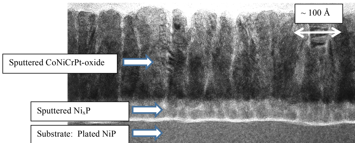
Cross-section TEM micrograph of Komag isotropic media showing its structure. (Figure 10-2)
