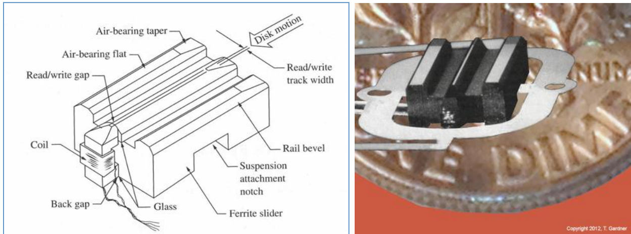
Schematic of ferrite head used in IBM 3340 drive, and photo of the head with the suspension. Dimensions: 4.0L x 3.2W x 0.86T mm. Photograph courtesy of Tom Gardner.
