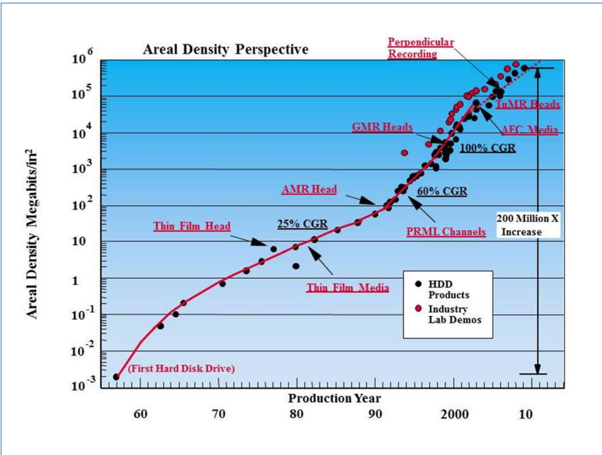
Areal density trend since the invention of HDD. Chart was created in 2010.
