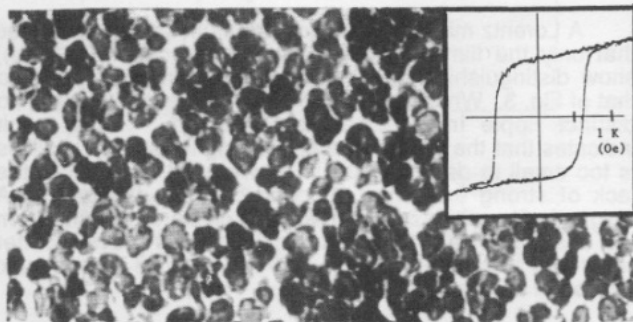
Fig. 6(b) Isolated particles, 50 μ (B-H loop insert)
