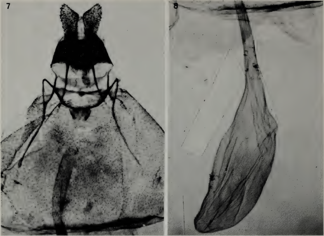
Figs. 7, 8. P. sandrinae g. & sp. n. 7, female genitalia, ovipositor and sterigma; 8, bursa copulatrix.
