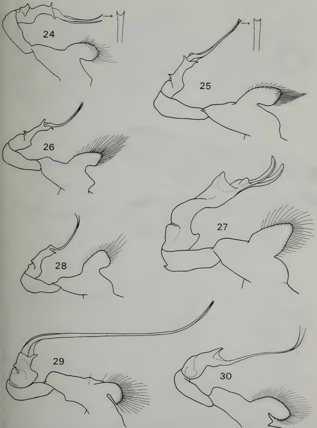
Figs. 24—30. Right profile view of penis in Phyllogomphoides : 24, fuliginosus , ♂ Surinam; 25, major , ♂ paratype Surinam; 26, cristatus , ♂ Surinam; 27, regularis , ♂ Santa Catarina, Brazil; 28, andromeda , ♂ Surinam; 29, undulatus , ♂ Surinam; 30, semicircularis , ♂ Colombia.
