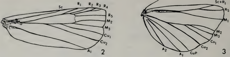
Figs. 2, 3. Forewing (2) and hindwing (3) venation of typical Roxita species.
