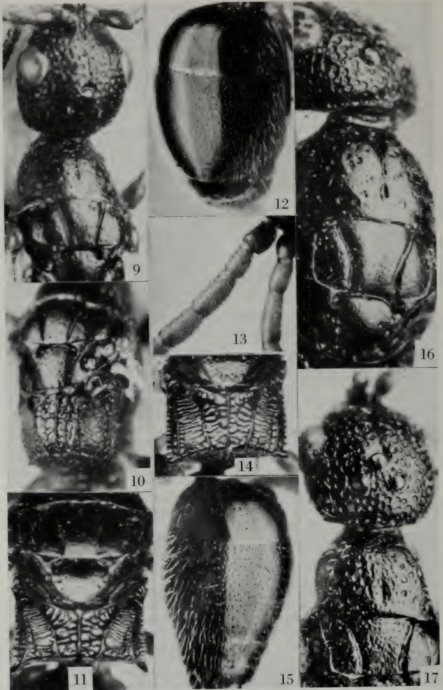
Figs. 9—10. Metrionotus bekeri sp. n., ♂, 9, head, pronotum and mesonotum; 10, scutellum and propodeum. Figs. 11—17. Heterocoelia nikolskajae sp. n. 11, scutellum and propodeum (♀); 12, abdomen (♀); 13, first antennal joints (♂); 14, propodeum (♂); 15, abdomen (♂); 16, head, pronotum and mesonotum (♀); 17, head, pronotum and mesonotum (♂).
