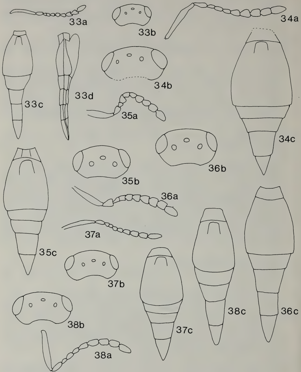
Figs. 33—38. a, antenna; b, head (dorsal view); c, metasoma (dorsal view); d, metasoma (lateral view). 33a—d, Platygaster chrysippus (lectotype); 34a—c, P. oculus (lectotype); 35a—c, P. gorge (lectotype); 36a—c, P. oebalus (paralectotype no. 296 in NMI); 37a—c, P. iolas (lectotype); 38a—c, P. demades (authors collection).
