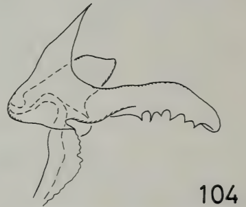
Figs. 100—104. N. hirsuticauda . Fig. 100. Hypopygium, lateral view. Fig. 101. Ovipositor, lateral view. Fig. 102. Extension of male tergite 9, dorsal view. Fig. 103. Left inner dististyle, from outside. Fig. 104. Adminiculum and left gonapophyses, lateral view.
