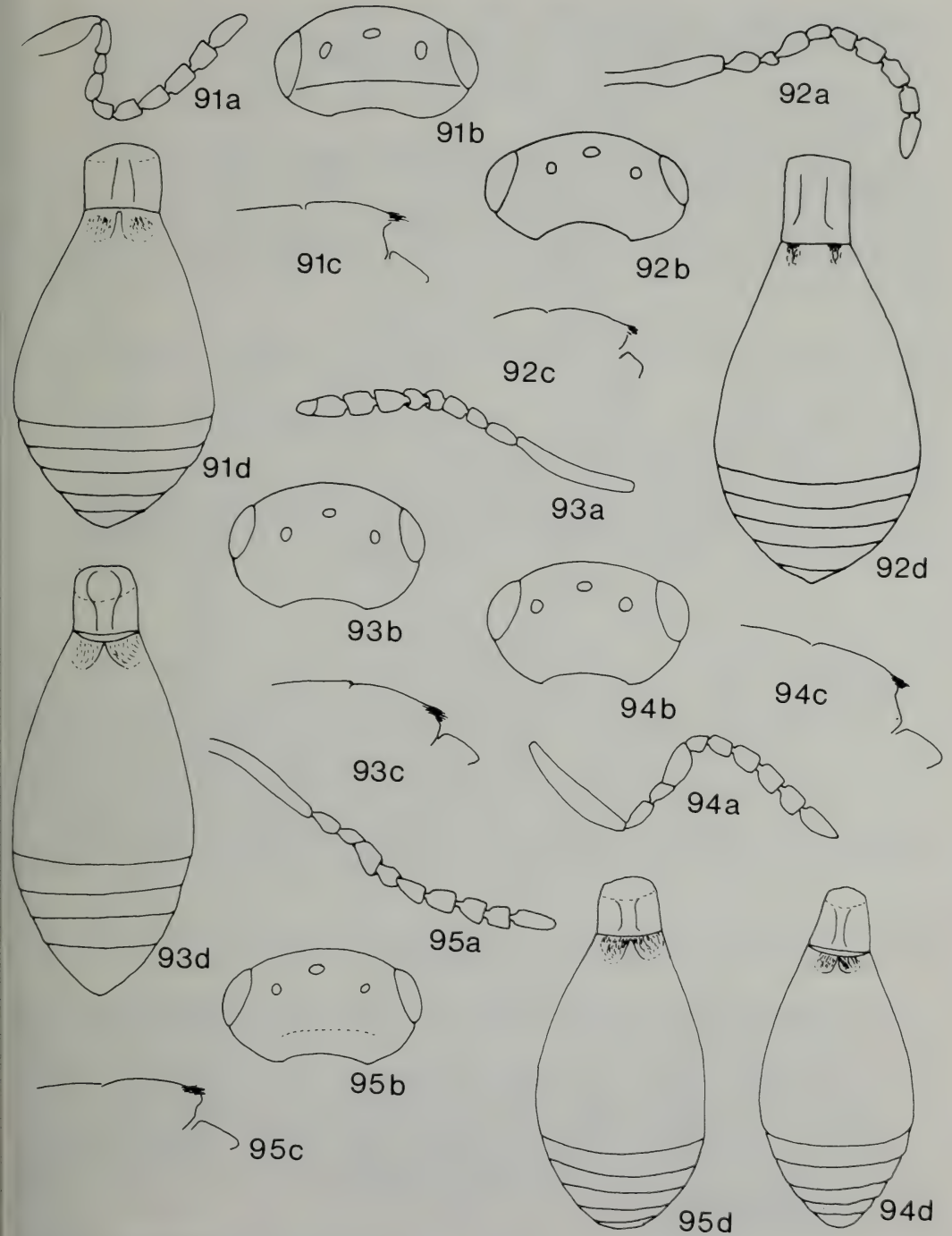
Figs. 91—95. a, antenna; b, head (dorsal view); c, scutellum (lateral view); d, metasoma (dorsal view). 91a—d, Amblyaspis tritici (lectotype); 92a—d, A. prorsa (lectotype); 93a—d, A. belus (lectotype); 94a—d, A. abas (lectotype); 95a—d, A. otrens (lectotype).
