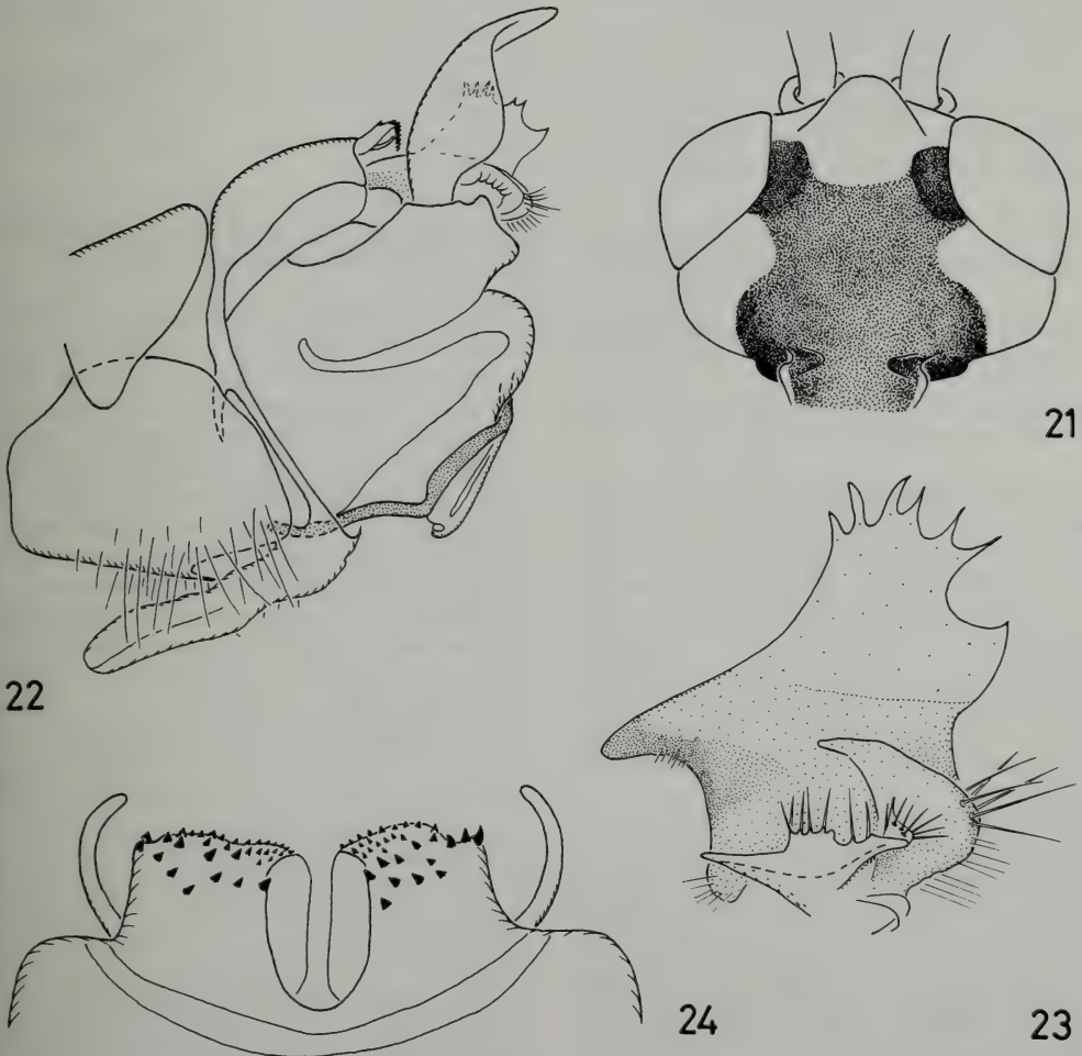
Figs. 21—24. N. daisensis . Fig. 21. Head, dorsal view. Fig. 22. Hypopygium, lateral view. Fig. 23. Left inner dististyle, from outside. Fig. 24. Extension of male tergite 9, dorsal view.
