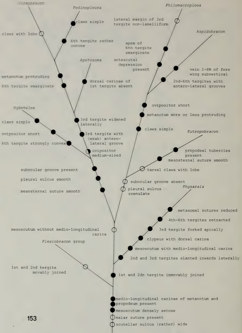
Fig. 153. Cladogram of the genera treated in this paper.
