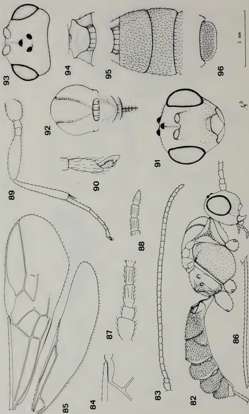
Figs. 82—96. Eutropobracon indicus Ramakrishna Ayyar, lectotype, ♀. 82, habitus, lateral aspect; 83, antenna; 84, vein 1-SR of fore wing; 85, wings; 86, ovipositor; 87, 1st—4th antennal segments, outer aspect; 88, apex of antenna; 89, hind leg; 90, outer hind claw; 91, head, frontal aspect; 92, mesosoma, dorsal aspect; 93, head, dorsal aspect; 94, 1st metasomal tergite, dorsal aspect; 95, 2nd and 3rd tergites, dorsal aspect; 96, 6th tergite, dorsal aspect. 82, 83, 85, 86, 89: scale-line (= 1 ×); 84, 87, 88, 90: 2.5 ×; 91, 93: 1.5 ×; 92, 94—96: 1.1 ×.
