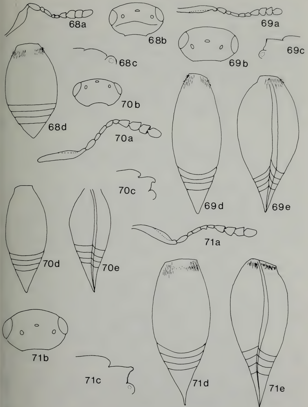
Figs. 68—71. a, antenna; b, head (dorsal view); c, scutellum (lateral view); d, metasoma (dorsal view); e, metasoma (lateral view). 68a—d, Synopeas euryale (lectotype); 69a—e, S. hyllus (lectotype); 70a—e, S. rbanis (lectotype); 71a—e, S. acco (lectotype).
