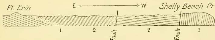
Section from Point Erin to Shelly Beach Point, showing connection between the two outcrops of grit: 1. Volcanic grit. 2. Sandstones and shales.
