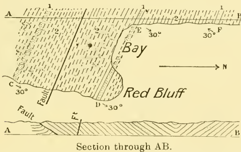
Plan and section showing connection between outcrops of volcanic grit at the Red Bluff: 1. Bands of volcanic grit. 2. Sandstones and shales. C, D, E, F. Four outcrops of grit.
