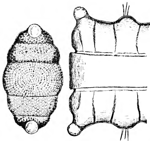
a. Fig. 197.— Biadulphia pulchella . a. Valve view. b. Girdle view.
