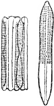
Fig. 91. Glyphodesmis Williamsonii . a. Girdle view. b. Valve view.
