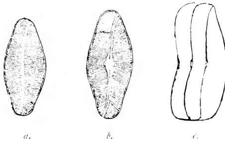
Fig. 60.— Achnanthidium flexellum . a, Upper valve. b, Lower valve. c, Frustule.
