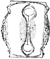
Fig. 148.— Goniothecium Odontella var. Danica .
