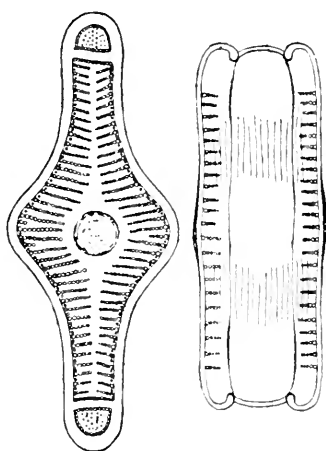
Fig. 92. Omphalopsis Australis Grev. a. Valve view. b. Girdle view.
