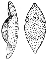
Fig. 186. Ploiaria petasiformis . a. Girdle view. b. Valve view.
