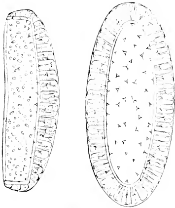
Fig. 160.— Muelleriella limbata . by keeping me au courant with his works.
