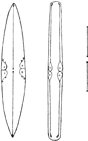
Fig. 28.— Stigmophora lanceolata , after Wallich.
