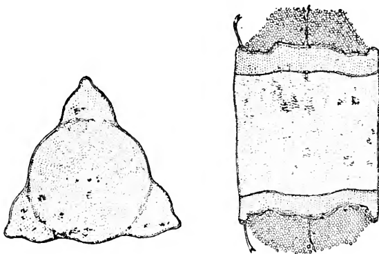
a. Fig. 196.— Lithodesmium undulatum . a. Valve view, b. Girdle view.
