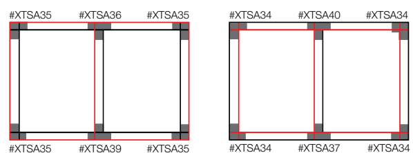
Three Circuit Floor View From Below
