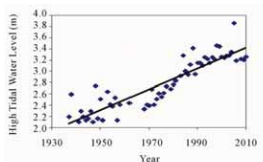
Figure 5.15: Trend in Annual Maximum High Tidal Water Levels at Rupsa-Pasur River (Mondal, 2012)
