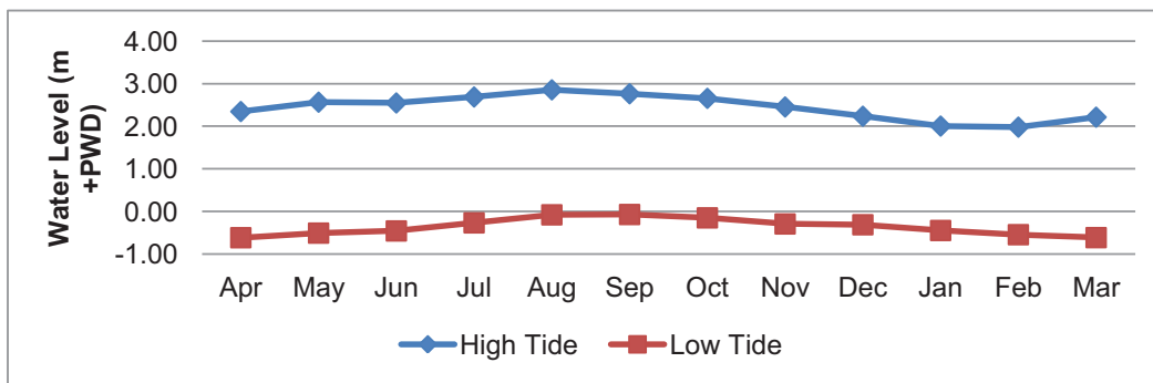
Figure 5.9: Surface Water Level at Chalna (Rupsa-Pasur River)
