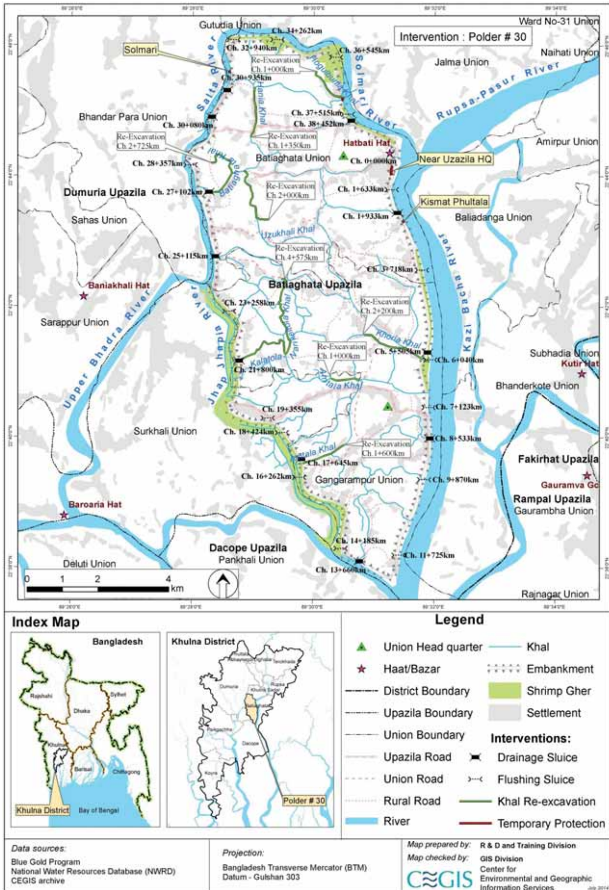
Map 4.1: Proposed Intervention Map of Polder 30
