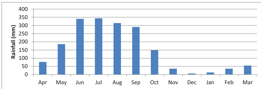
Figure 5.1: Average Monthly Rainfall at Khulna BMD
