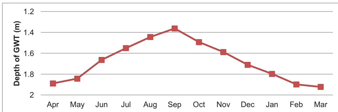
Figure 5.10: Average Monthly Variations of Ground Water Table
