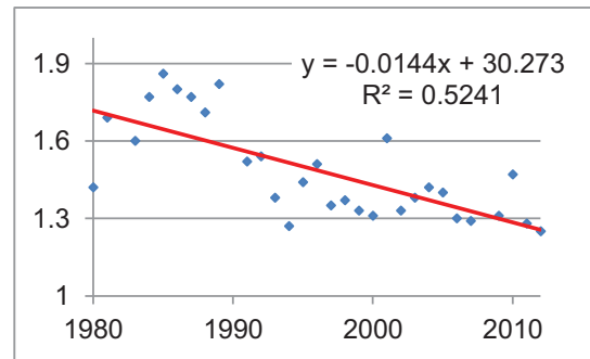
Figure 5.12: Variation of GWT at KHU003 in September (1980 – 2013)
