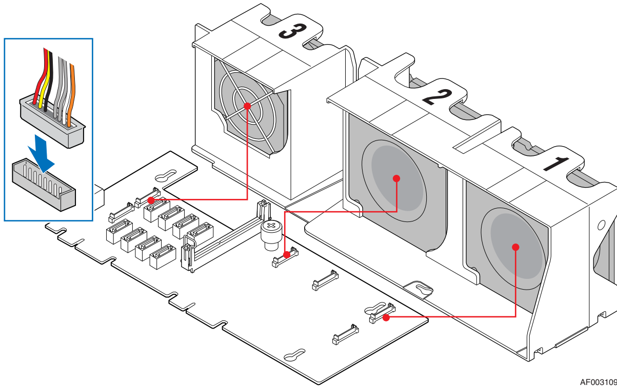
Figure 15. Non-redundant Fan Header Assignments on Midplane
