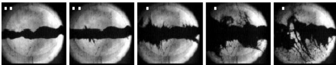
Figure 4. Pictures of the mercury jet disintegrating when hit by the proton beam. No magnetic field. Exposures of 25\ \mu\text{s} at t = 0, 0.75, 2, 7, 18\text{ ms} after a 1 cm diameter mercury jet was struck by a pulse of 2 \times 10^{12} protons at 24 GeV.
