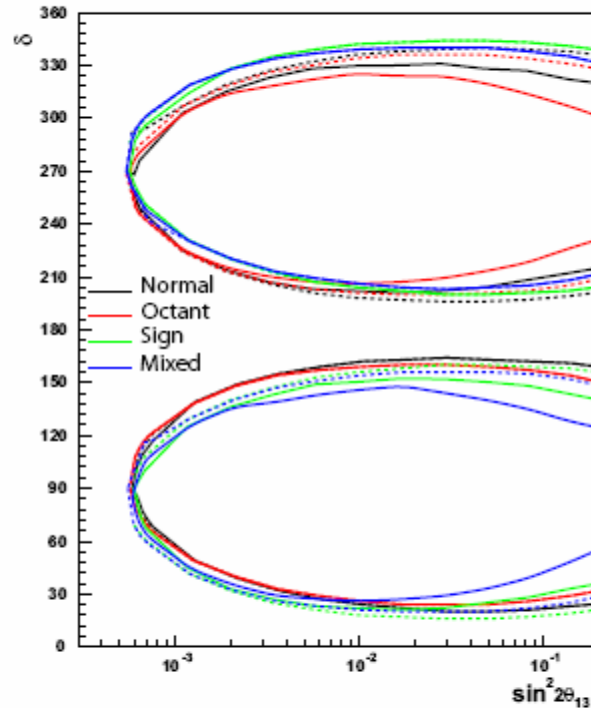
Figure 11: Leptonic CP violation discovery potential at 3\sigma ( \Delta\chi^2 > 9.0 ) of the BetaBeam with \gamma = 100 computed for the 4 different options about the true values of \text{sign}(\Delta m_{23}^2) and \theta_{23} and including all the possible degeneracies (see text). Dotted curves are computed neglecting the effects of the clone solutions. Taken from ref. [107]
