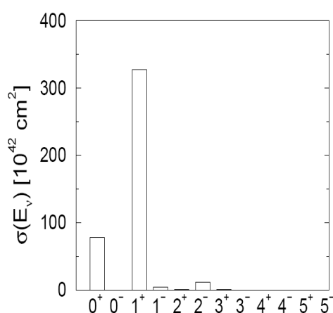
Figure 1 Contribution of the states of different multipolarity to the total charged-current \nu_e - ^{48}\text{Ca} cross section for neutrino energy E_\nu = 30 MeV. The histograms show the contribution of the Fermi ( J^\pi = 0^+ ), the Gamow-Teller ( 1^+ ) and the spin-dipole ( 0, 1, 2^- ) states and all higher multipoles up to 5 [vol05].
