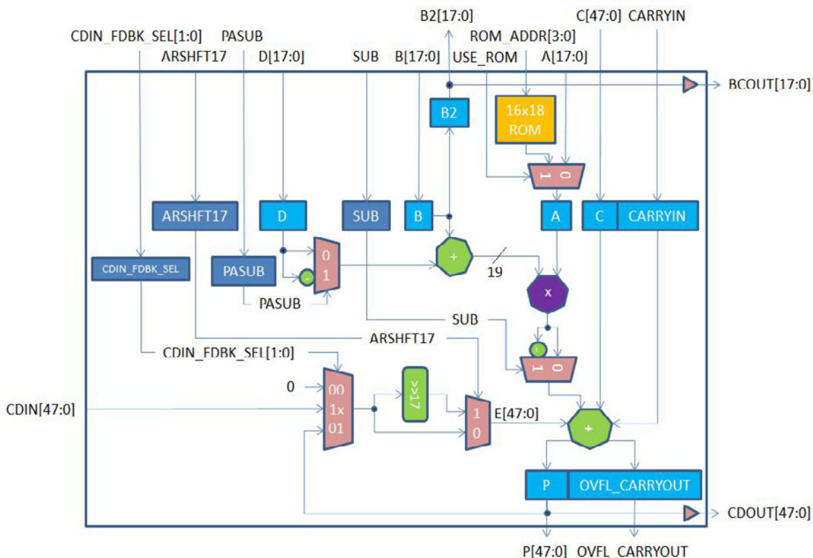
Figure 59 • Simplified Block Diagram of MACC_PA
