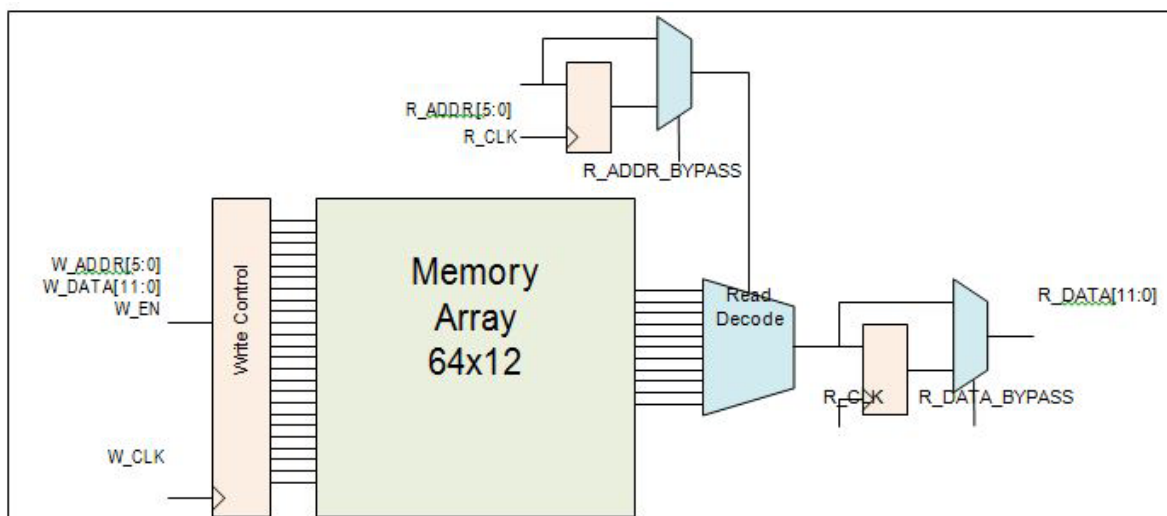
Figure 57 • Simplified Block Diagram of RAM64x12
