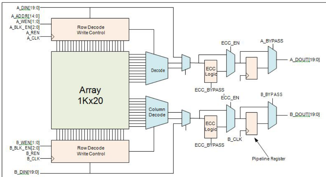
Figure 56 • Simplified Block Diagram of RAM1K20
