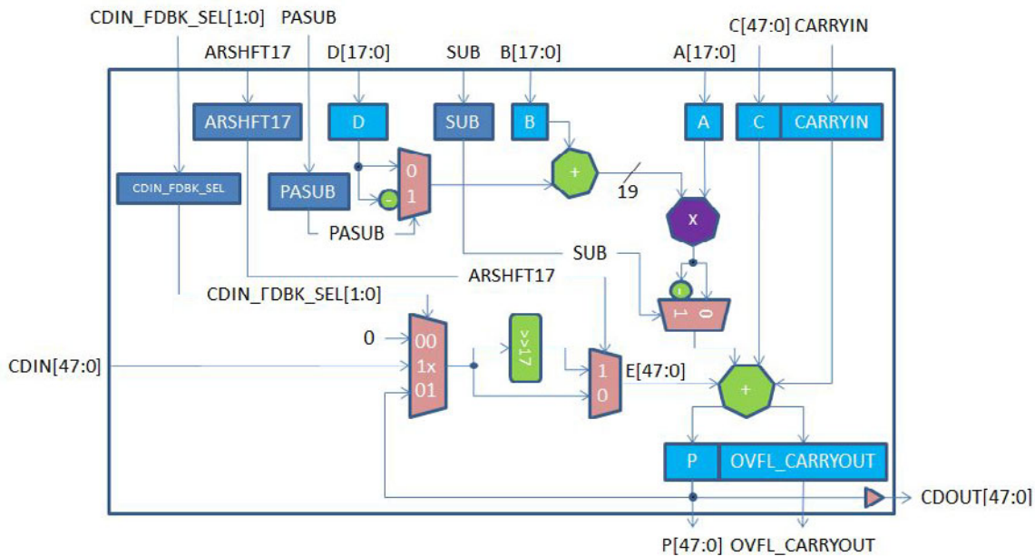
Figure 58 • Simplified Block Diagram of MACC_PA
