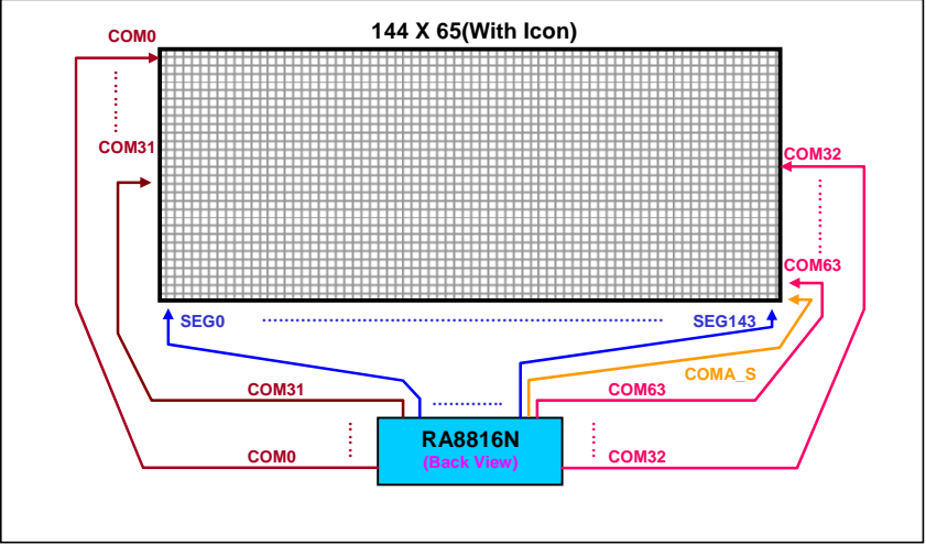
Figure A- 5 : The Connection of RA8816N with LCD Panel (144x65)
