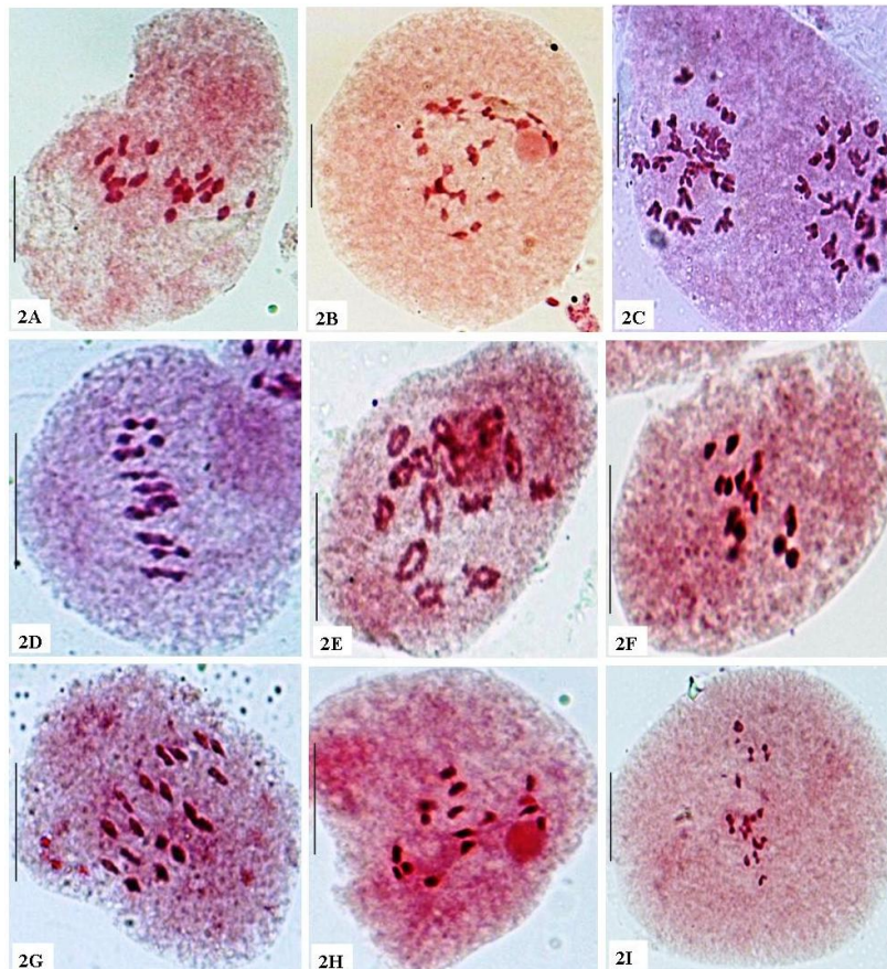
Figure Plate 2: 2A P. purpureum - PMC at M-I showing 18_{II} . 2B P. purpureum - PMC at diakinesis showing 21_{II} . 2C Phalaris minor - PMC at M-II showing 21: 21 chromosomes. 2D Pogonatherum crinitum - PMC at M-I showing 10_{II} . 2E P. crinitum - PMC at diakinesis showing 14_{II} . 2F Setaria barbata - PMC at M-I showing 16_{II} . 2G S. barbata - PMC at M-I showing 18_{II} . 2H S. homonyma - PMC at diakinesis showing 16_{II} . 2I Monochoria vaginalis - PMC at M-I showing 12_{II} . Scale= 10\mu\text{m}
