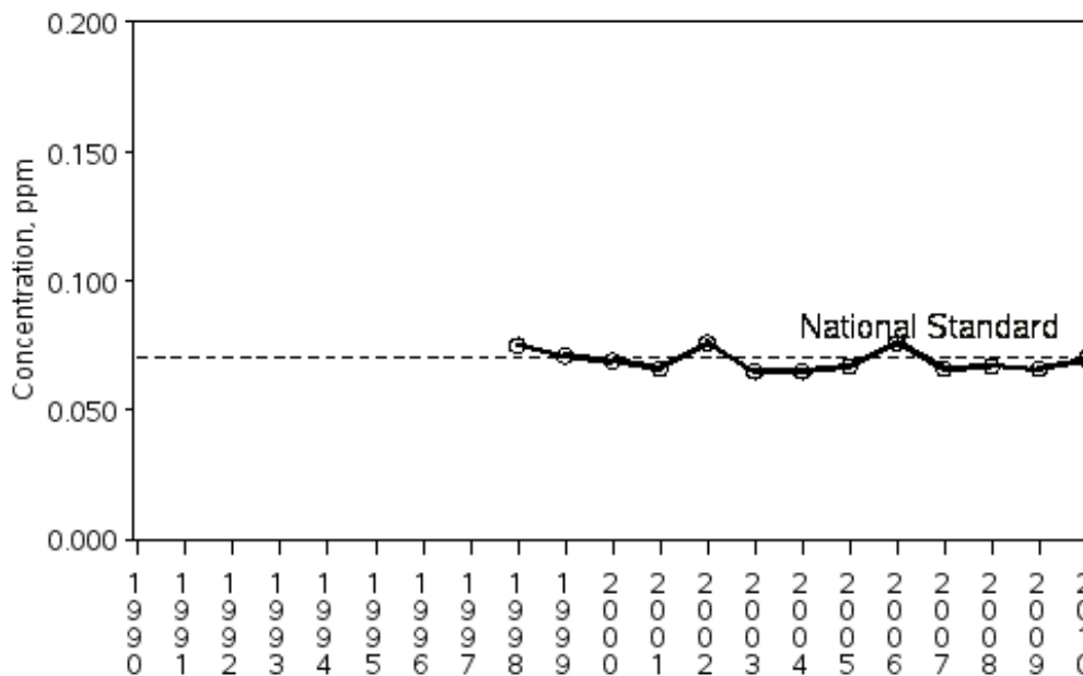
Figure 19. Average annual ozone (O 3 ) concentration (ppm) for the GUMO region, 1998-2010 (EPA 2012), compared to the national standard of 75 ppb that became effective in 2008. Note: Site 350151005 is the monitor located in Carlsbad, New Mexico, approximately 80 km (50 miles) northeast of GUMO.
