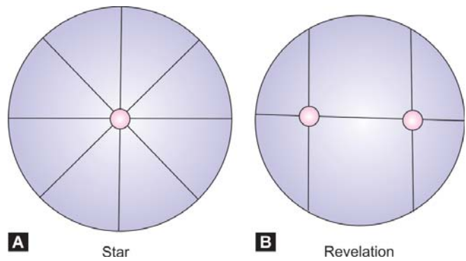
Figs 5.60A and B: Flute end designs; (A) Star, (B) Revelation
