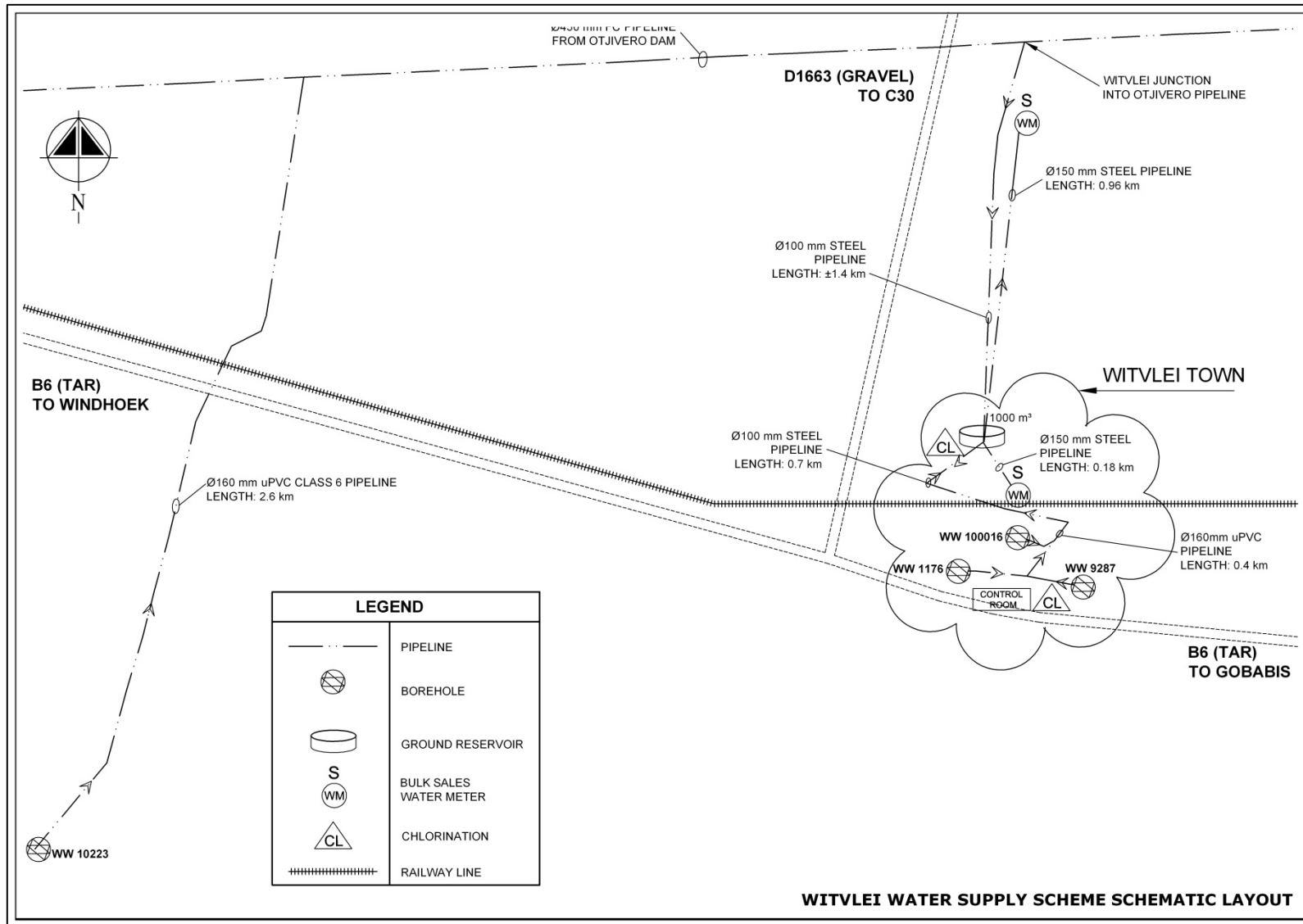
Figure 1: Witvlei Scheme Layout
