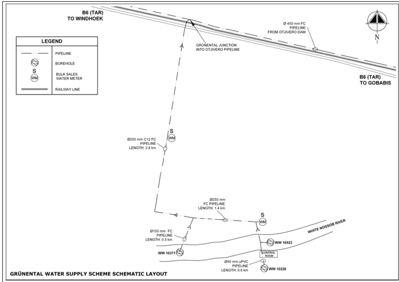
Figure 2: Grünental Scheme Layout
