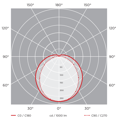
771-Favourite LED 39 W (Prevaled)
