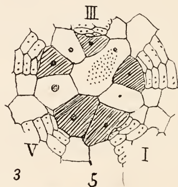
FIG. 3.— Micraster coranquineum (Lam.). Cretaceous, England. \times 6.7 . Oculars I, V meet and cover ambulacra I, V and interambulacrum 5. (After Jackson, 1912, fig. 174, p. 149.)
