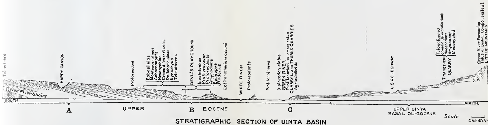
STRATIGRAPHIC SECTION OF UINTA BASIN
