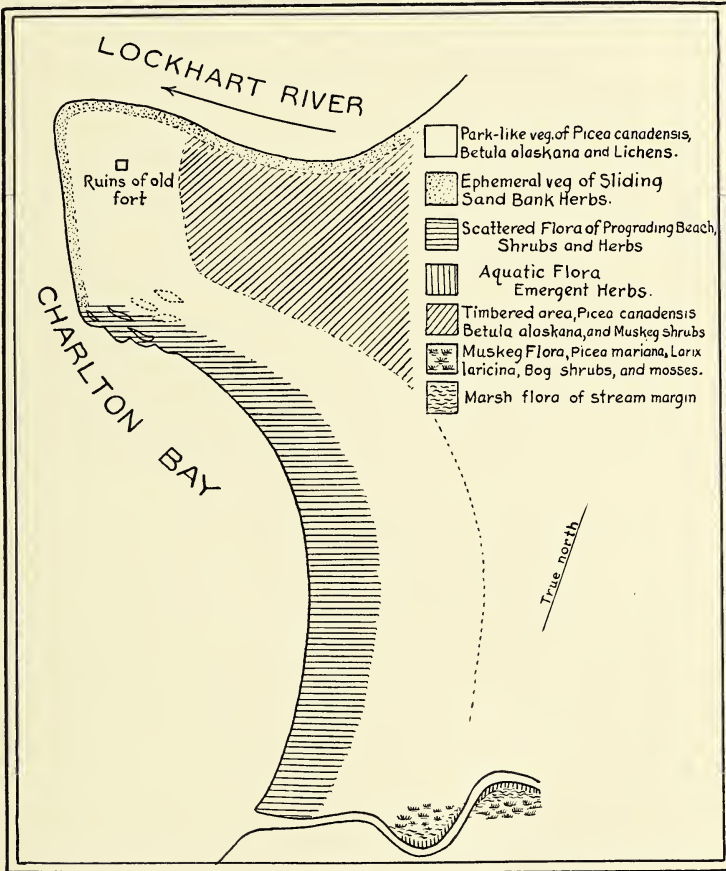
Fig. 2. Distribution of Vegetation.
