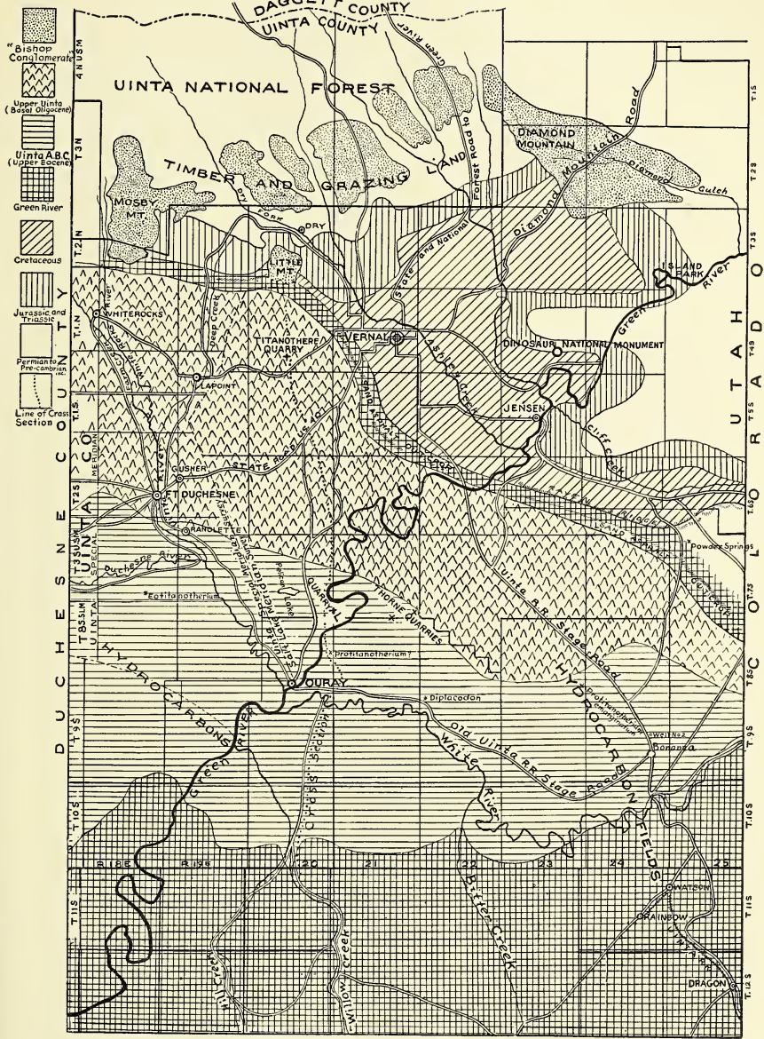
GEOLOGICAL MAP OF EASTERN UTAH BASIN
