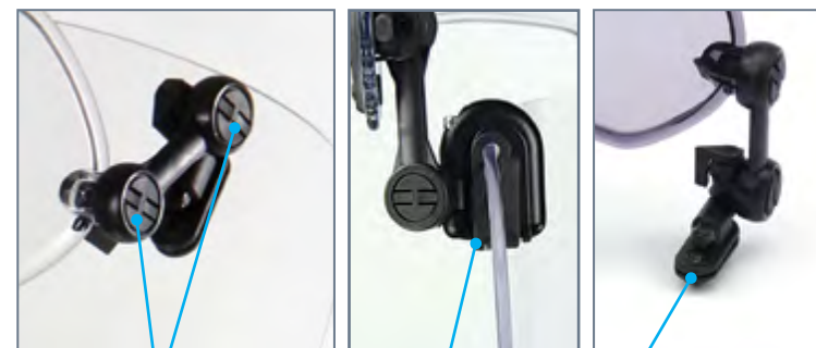
Dual pivots allow height and angle adjustments.
