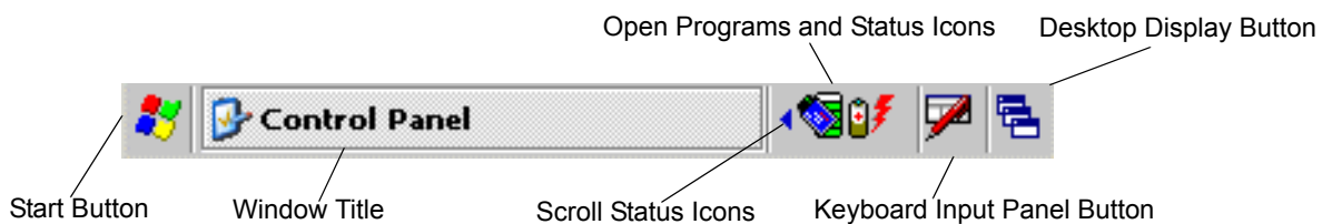
Figure 2-7 Taskbar
