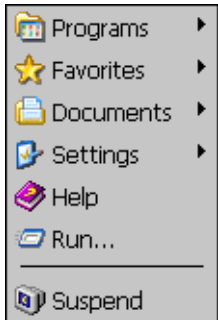
Figure 2-8 Start Menu
