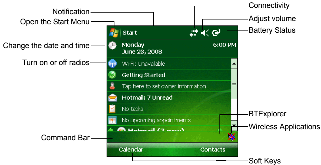
Figure 2-14 Today Screen
