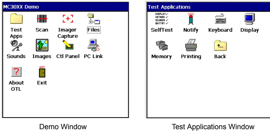
Figure 2-5 Demo Window
