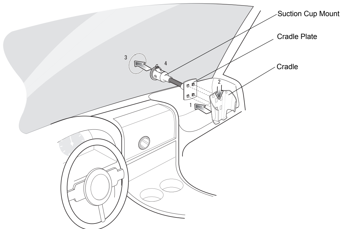
Figure 6-13 Windshield Installation
