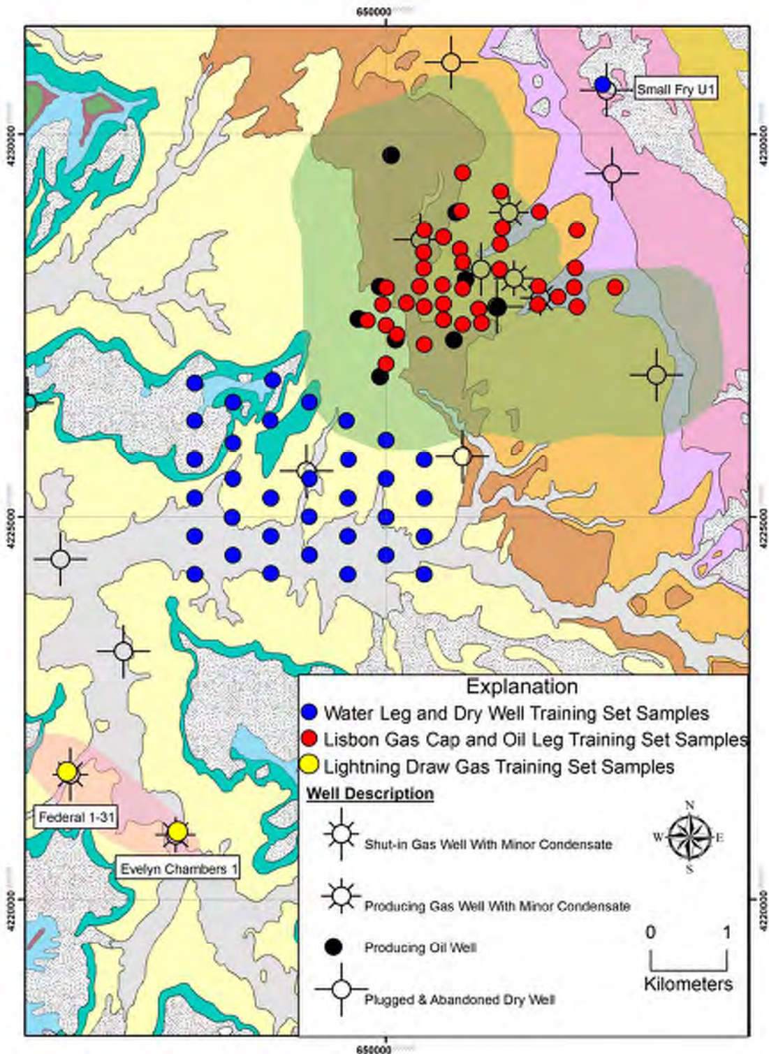
Figure 5-21. Surface soil training set samples used for two component Lisbon gas cap/ oil leg versus water leg and Lightning Draw Southeast gas versus Lisbon water leg discriminant analysis models. See figure 5-11 for description of geologic units (geologic base modified from Doelling, 2005). Lisbon and Lightning Draw southeast fields shown in bluish green and pink, respectively.
