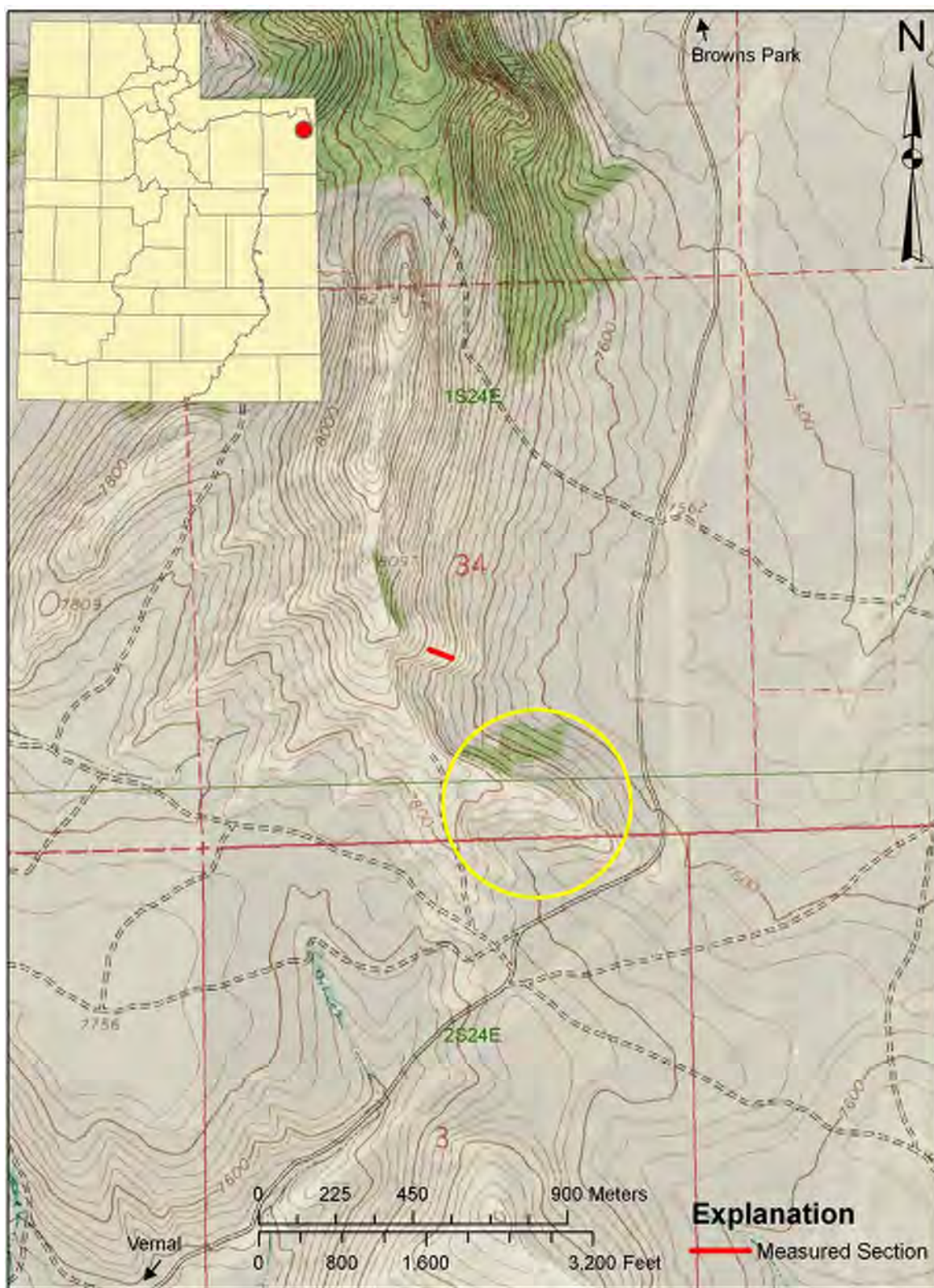
Figure 8-15. Location of Crouse Reservoir/Diamond Mountain Plateau study site (key brecciated outcrop indicated with yellow circle). Base map: Crouse Reservoir 1:24,000 topographic quadrangle map, U.S. Geological Survey.
