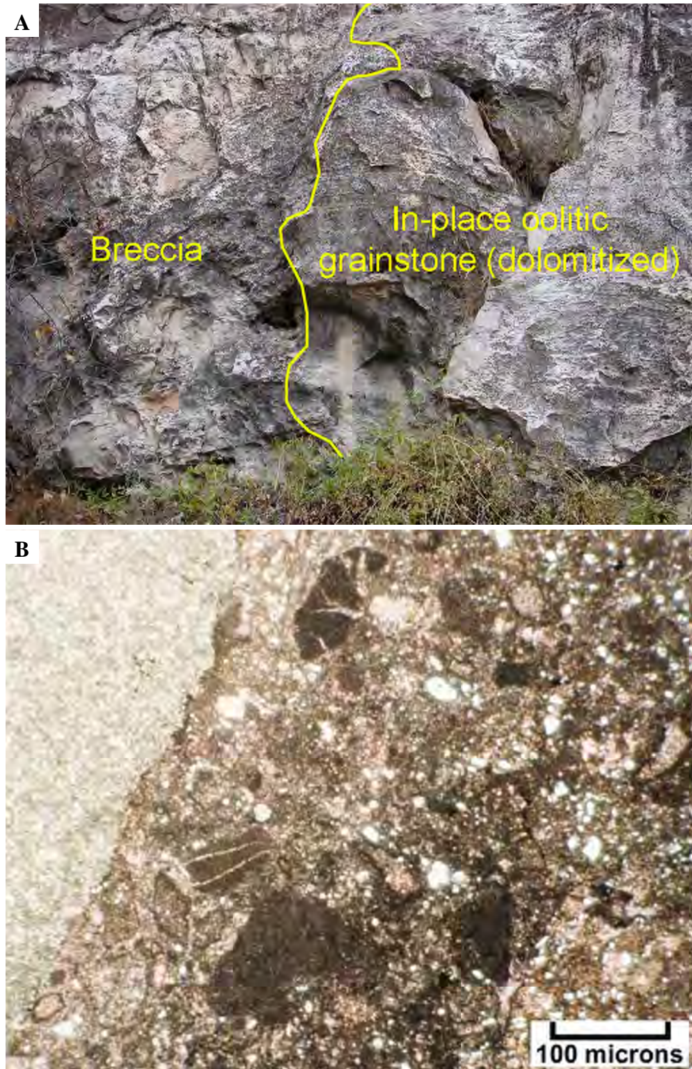
Figure 8-13. Megabreccia in study site 2. A – Small-scale oolitic shoal and collapse breccia (outcrop is approximately 10 feet [3 m] high). B – Photomicrograph (plane light) showing the contact between dolomitic grainstone (light gray, upper left) and the dolomitized karst cavity filling of small carbonate clasts.
