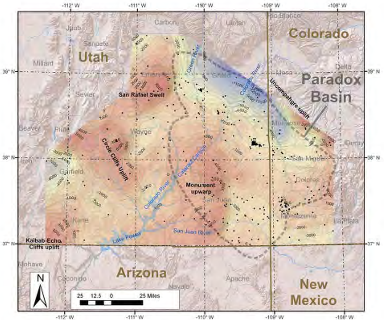
Figure 11-4. Structural contours on the top of the Leadville Limestone derived from oil and gas exploration wells. Note that the contours do not consider fault offsets and folding between the wells. The contour interval is 1000 feet (relative to sea level). The structural highs correspond to Laramide uplifts.
