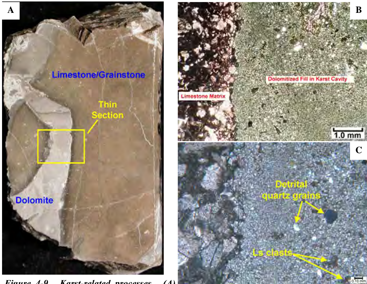
Figure 4-9. Karst-related processes. (A) Conventional core slab of a limey, oolitic, peloidal/skeletal grainstone with a dolomitized sediment-filled cavity. (B) Low-magnification photomicrograph (plane light) showing the contact between the non-porous limestone matrix and the non-porous dolomitized and siliciclastic karst cavity filling. (C) Photomicrograph (cross-polarized light) showing the contact between limestone matrix and the dolomitized karst cavity filling; note that the dolomitized filling is composed of very fine crystals. (D) Higher magnification photomicrograph (plane light) of detrital quartz grains (white) and small carbonate clasts (dark gray) within the tight, dolomitized mud filling the karst cavity. Lisbon No. D-616 well (figure 2-1), 8308-8309 feet, porosity = 1.2%, permeability = 11.1 mD.
