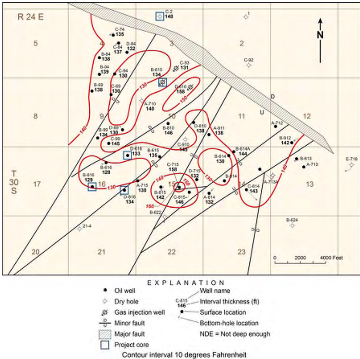
Figure 2-12. Bottom-hole temperature map, Leadville Limestone, Lisbon field.
