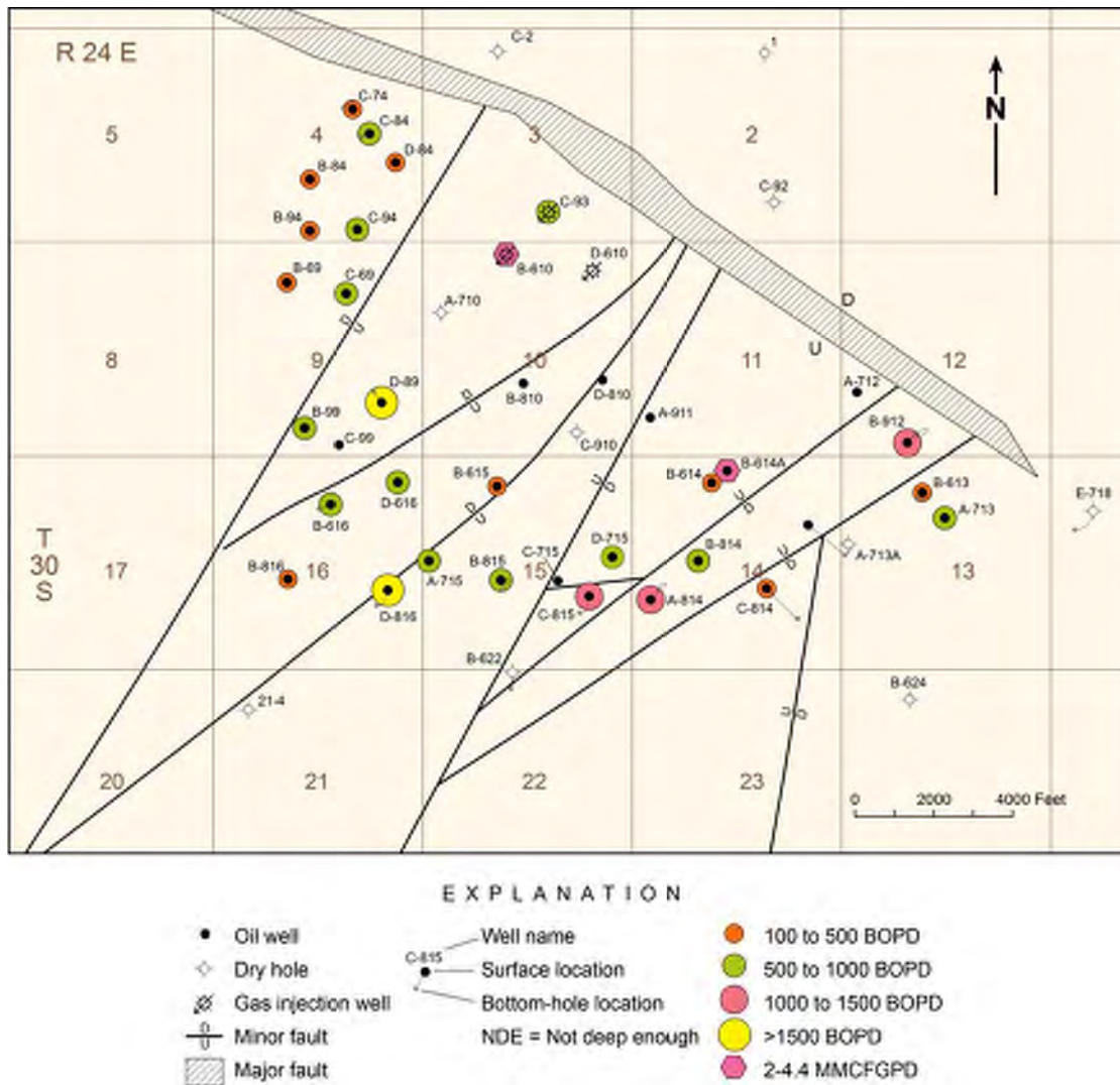
Figure 2-13. Initial flowing potential, Leadville Limestone, Lisbon field.
