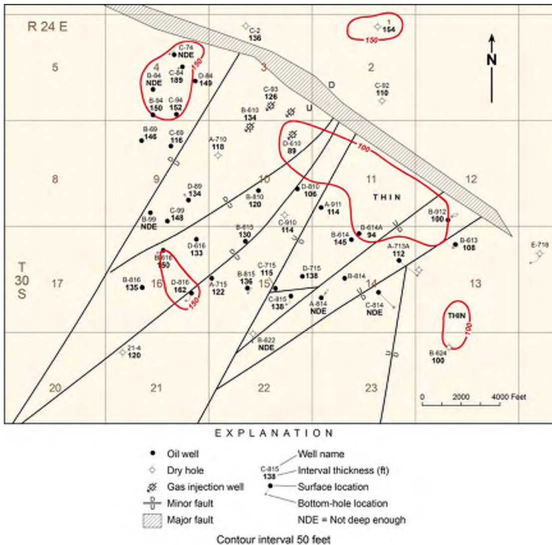
Figure 2-5. Isochore of zone 2, Leadville Limestone, Lisbon field.
