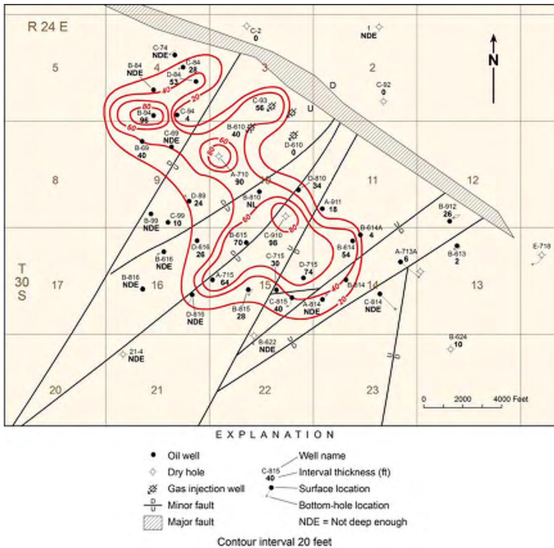
Figure 2-10. Net feet of porosity isochore for reservoir zone 3, Leadville Limestone, Lisbon field.
