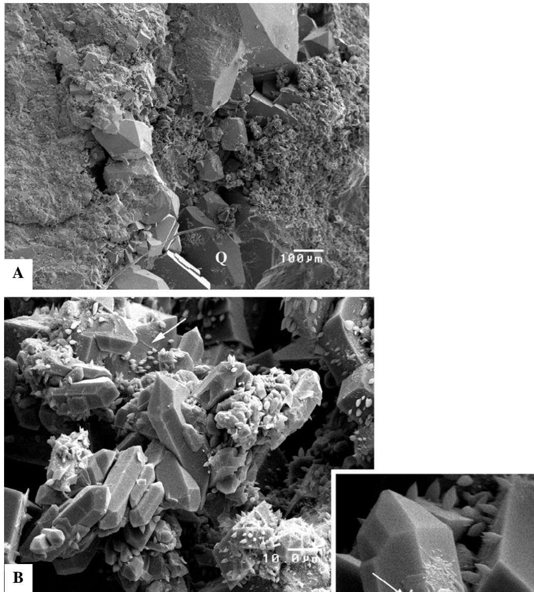
Figure 4-23. Scanning electron microscope photomicrograph showing euheedral quartz void fillings (Q) within late dissolution pores. A – Typical euheedral quartz surrounded by rhombic dolomite; core plug from 8356 feet, Lisbon No. D-616 well. Scale bar represents 100 microns (0.1 mm). No core-plug analysis available. B – Core plug from 8486 feet, Lisbon No. D-816 well, showing showing clusters of euheedral, doubly terminated quartz crystals (“miniherkimers”). The small spiky materials precipitated on many of the surfaces are either pyrobitumen or sulfide minerals. Scale bar represents 10 microns (0.01 mm). Porosity = 5.9%; permeability = 0.2 mD based on core-plug analysis. C - Closeup of a typical doubly terminated quartz crystal from same core sample in B. The linear features (arrow) and the spiky materials on many of the crystal surfaces are composed of either pyrobitumen or sulfide minerals.
