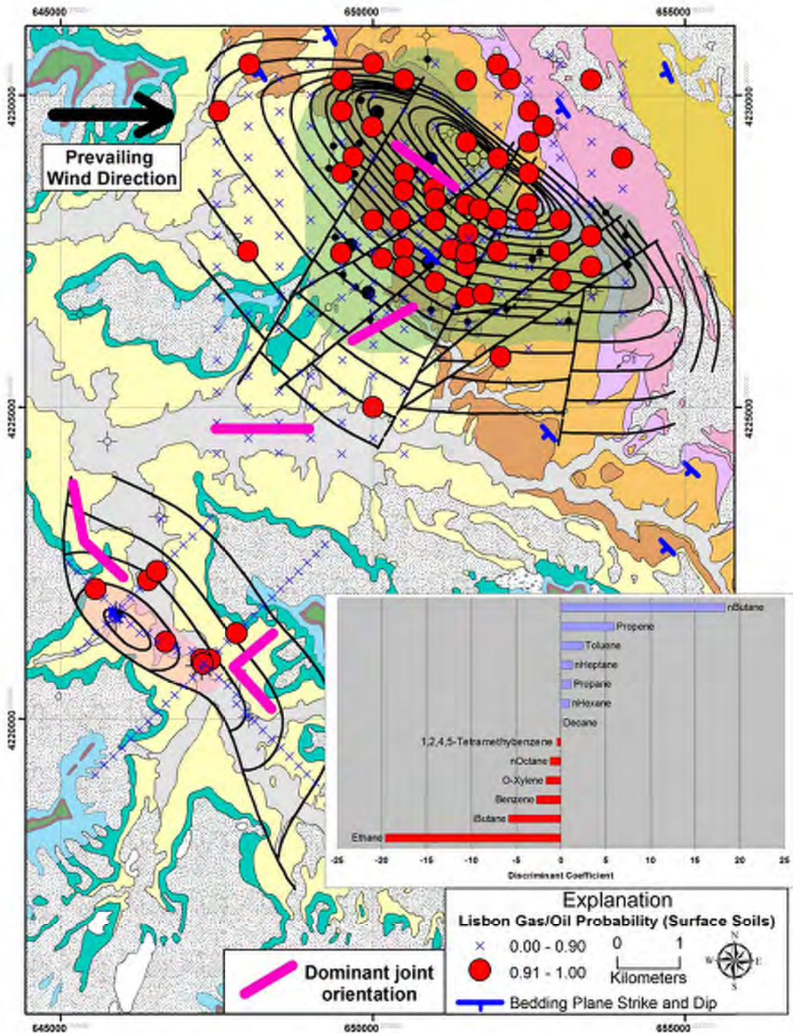
Figure 5-22. Distribution of Lisbon gas-oil probabilities derived from two-component discriminant analysis of thermally desorbed C 1 to C 12 hydrocarbon from surface soils. See figure 5-11 for description of geologic units (geologic base modified from Doelling, 2005) and figure 5-1 for explanations of well symbols; form line contours based on structure contour maps of the Leadville Limestone shown on figures 5-1 and 5-5. Lisbon and Lightning Draw southeast fields shown in bluish green and pink, respectively.
