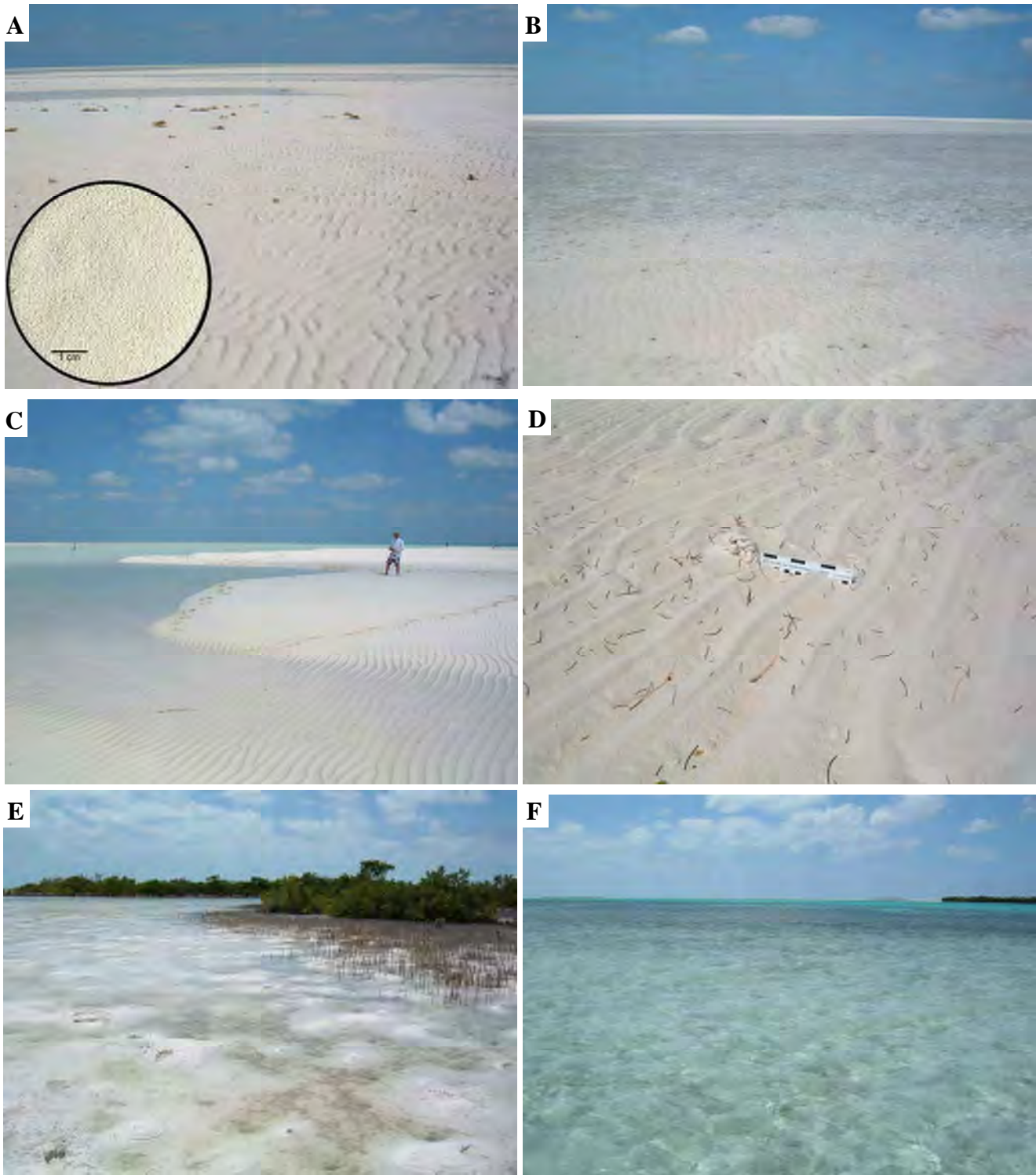
Figure 9-30. Joulter's Cay ooid shoal complex. A – Ooid shoals as far as the eye can see (view to the north). Flat topped current ripples due to flood-tidal currents. Inset is closeup of typical Joulter's Cay ooids. B – Slightly flooded ooid shoals forming bi-directional current ripples. C – Shallow tidal pools and rippled, exposed shoals of ooids (cross-bedded). D – Small burrow by the bivalve Tivela abaconia in rippled ooid sediments. E – Stabilized grain flats composed of ooids and peloids, colonized by red mangroves. Note numerous active Callianassa burrows. F – Tidal channel that leads to northeasterly directed ebb-tidal delta.
