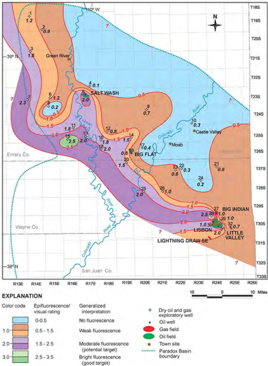
Figure 6-6. Map of the highest average epifluorescence based on visual rating of well cuttings, Paradox fold and fault belt, Utah.
