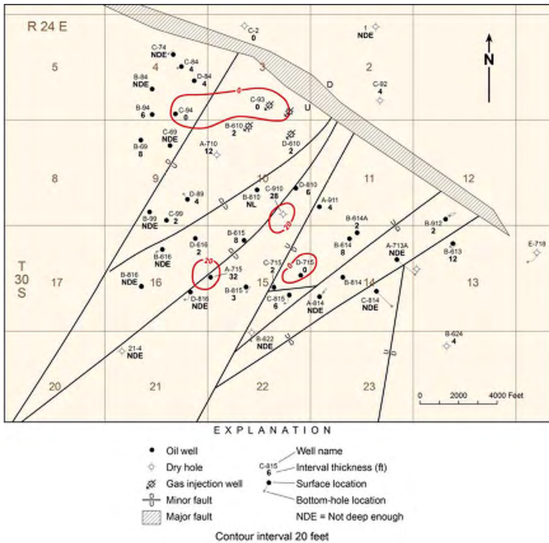
Figure 2-11. Net feet of porosity isochore for reservoir zone 4, Leadville Limestone, Lisbon field.
