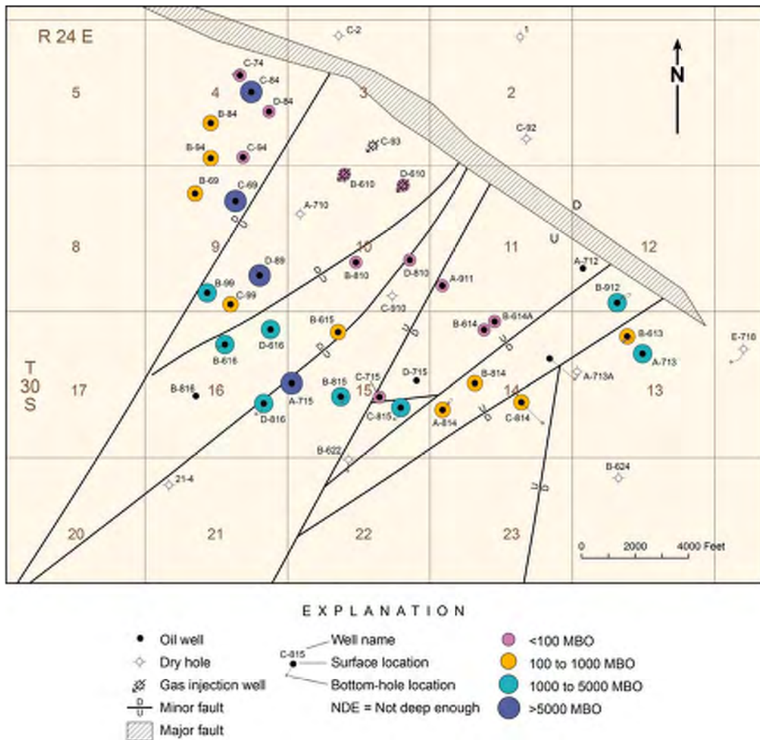
Figure 2-14. Cumulative oil production, Leadville Limestone, Lisbon field.
