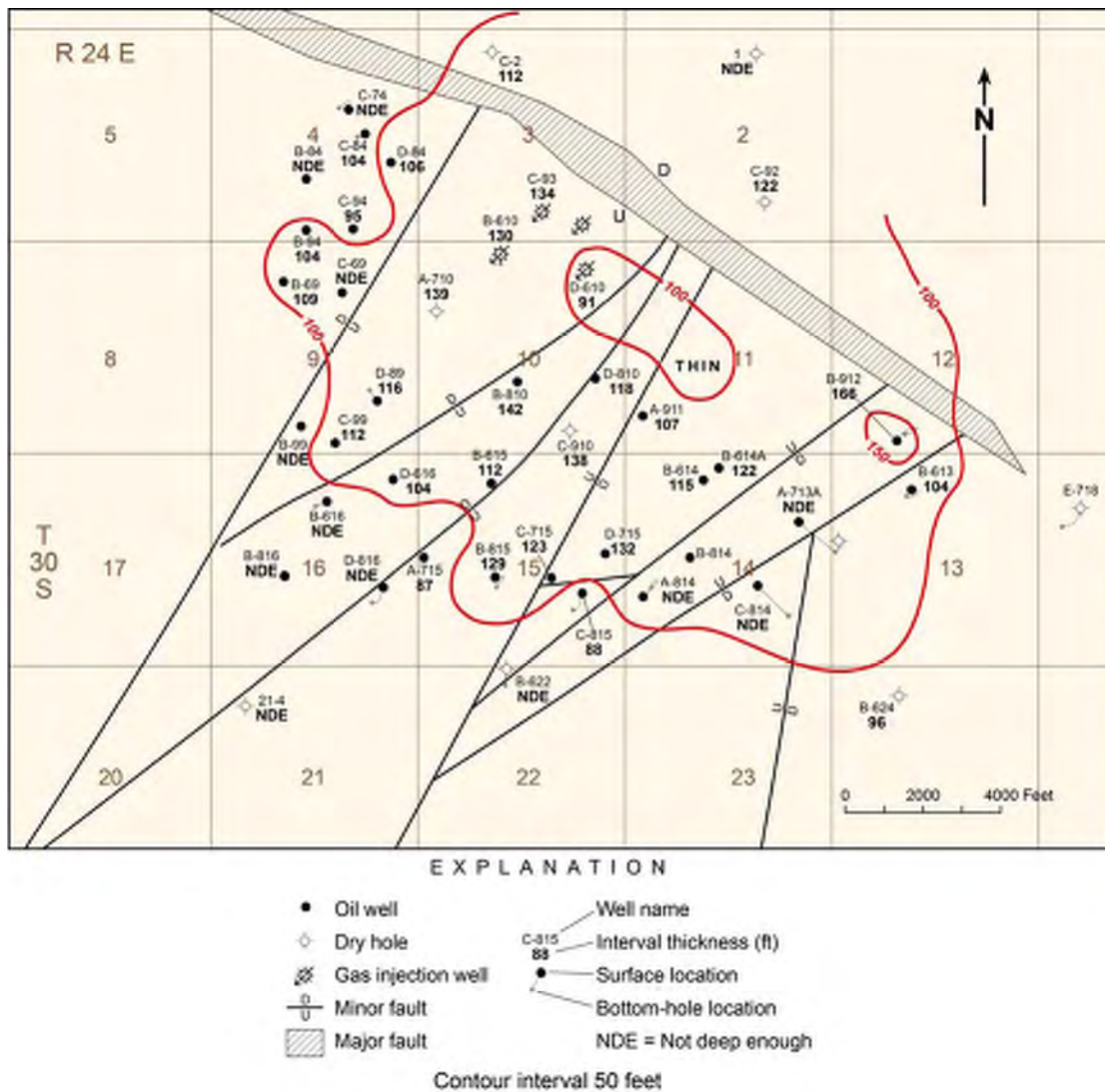
Figure 2-6. Isochore of zone 3, Leadville Limestone, Lisbon field.
