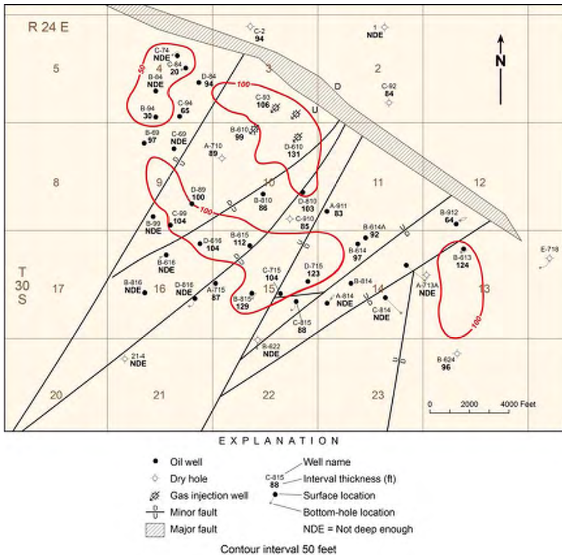
Figure 2-7. Isochore of zone 4, Leadville Limestone, Lisbon field.
