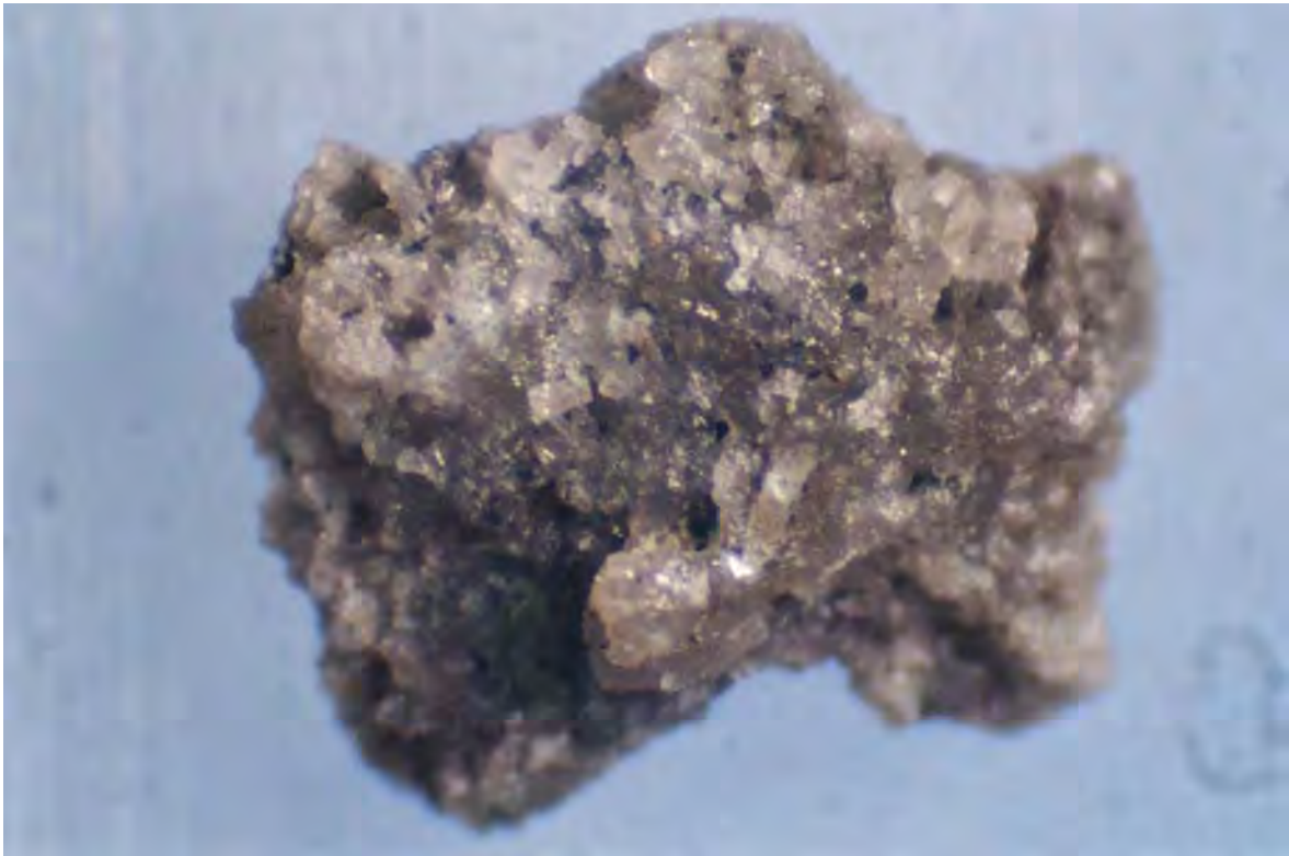
Binocular microscope image (4500x) – Pure Lisbon 814-A (Map #31), 8900-05 feet, single dolomite cutting with intercrystalline porosity and traces of bitumen.
