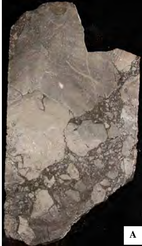
Figure 4-6. (A) Conventional core slab showing a dolomite “autobreccia” in which the clasts have moved very little. The black material surrounding the in-place clasts is composed of porous late dolomite coated with pyrobitumen. (B) Entire thin section overview from the core in A, showing low-porosity, white dolomite clasts surrounded by solution-enlarged fractures partially filled with coarse rhombic (RD) and saddle dolomites that are coated with pyrobitumen (bit). These black areas between the clasts exhibit very good intercrystalline porosity. The open fracture segments (in blue) between clasts are bridged by coarse, saddle dolomite cements (SDC). (C) Entire thin section overview from the core in A, of black, porous, dolomite clasts surrounded in this case by coarse, low-porosity saddle dolomites. These white dolomites were probably early dolomite (ED) filling space between possible “hydrofractured” replacement dolomites. The black porous dolomites are mostly rhombic (planar) dolomites (RD) coated with thin films of pyrobitumen (bit). Lisbon NW USA No. B-63 well (figure 2-1), 9938.3 feet, porosity = 6.4%, permeability = 54 mD.
