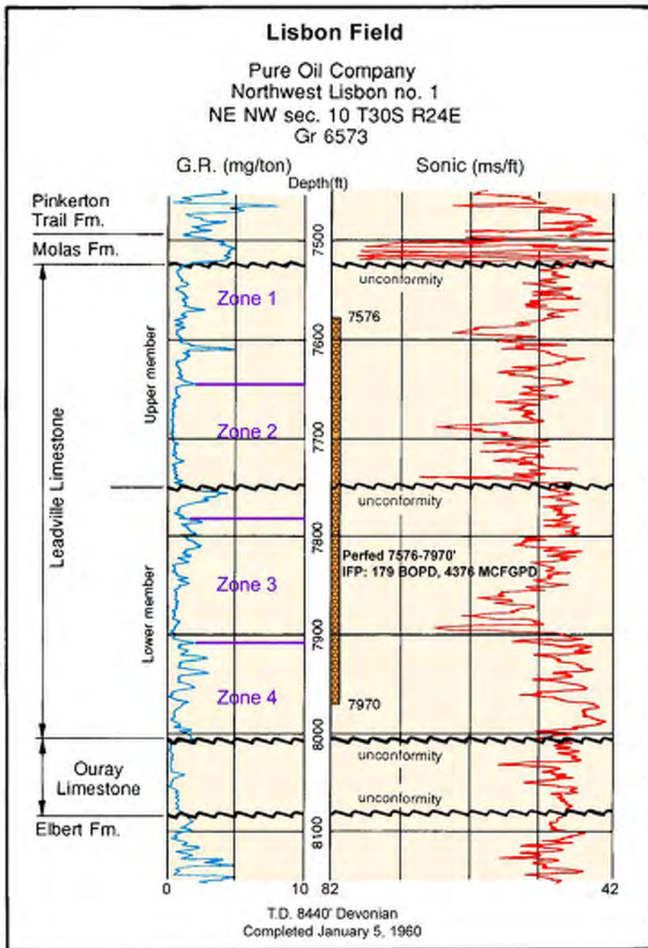
Figure 2-3. Typical gamma ray-sonic log of the Leadville Limestone showing the four reservoir zones defined in this study; Lisbon field discovery well, San Juan County, Utah. See figure 2-1 for well location.
