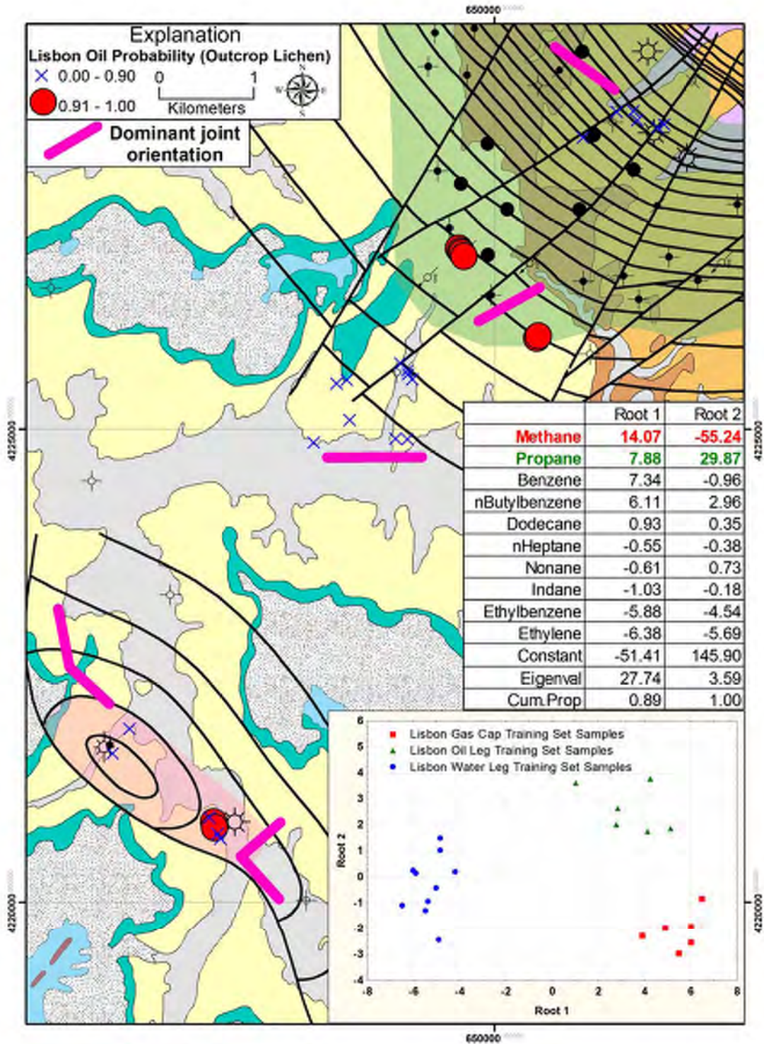
Figure 5-26. Distribution of Lisbon oil probability derived from three-component discriminant analysis of thermally desorbed C 1 to C 12 hydrocarbon from outcrop lichen samples. See figure 5-11 for description of geologic units (geologic base modified from Doelling, 2005) and figure 5-1 for explanations of well symbols; form line contours based on structure contour maps of the Leadville Limestone shown on figures 5-1 and 5-5. Lisbon and Lightning Draw southeast fields shown in bluish green and pink, respectively.
