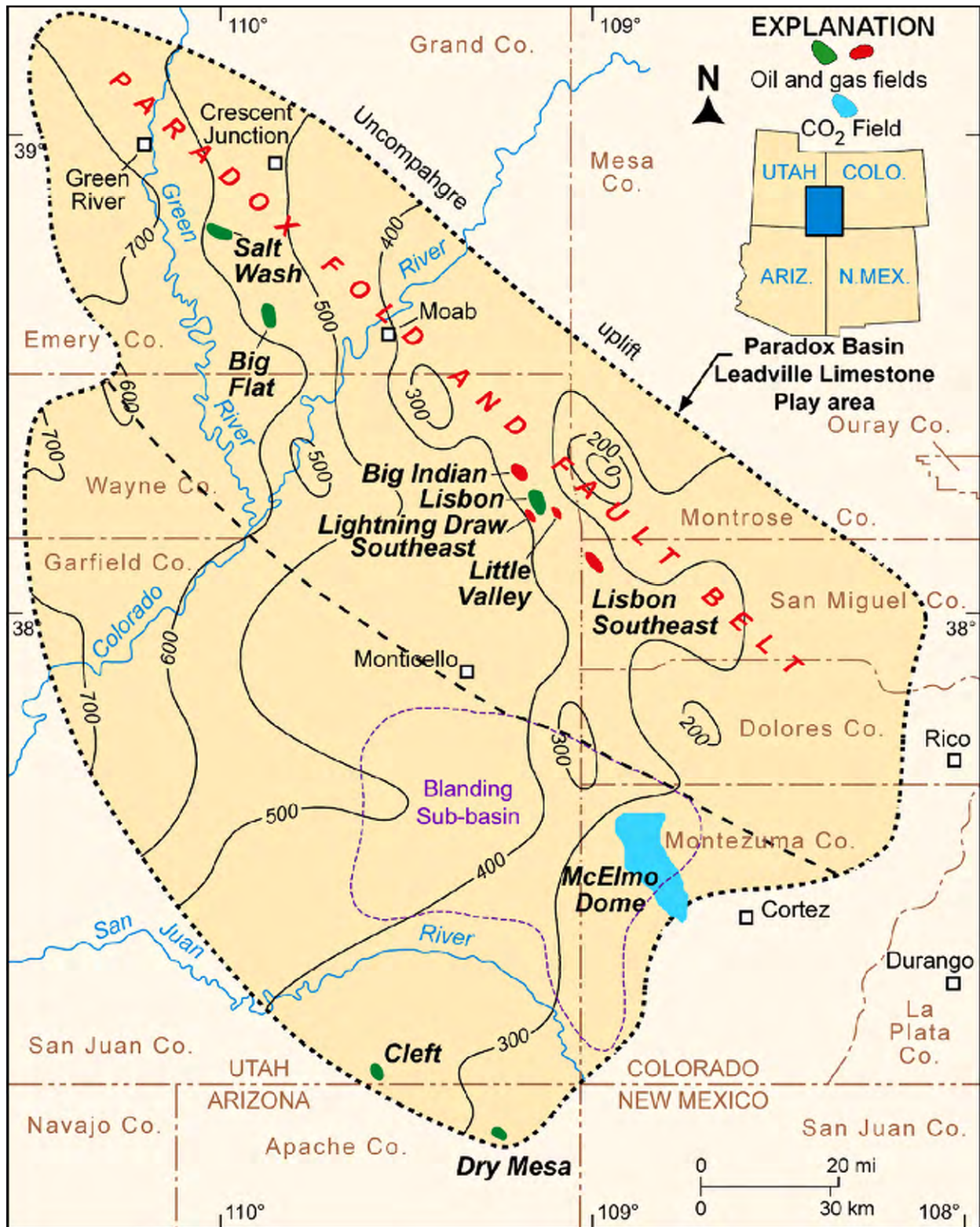
Figure 1-3. Regional setting of the Paradox Basin, showing oil and gas fields that produce from the Mississippian Leadville Limestone, and thickness of the Leadville (contour interval is 100 feet). Modified from Parker and Roberts (1963).
