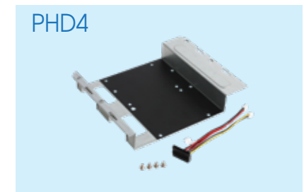
PHD4 XH170V/XH110V 3.5" hard drive rack for 3-liter Slim PCs
