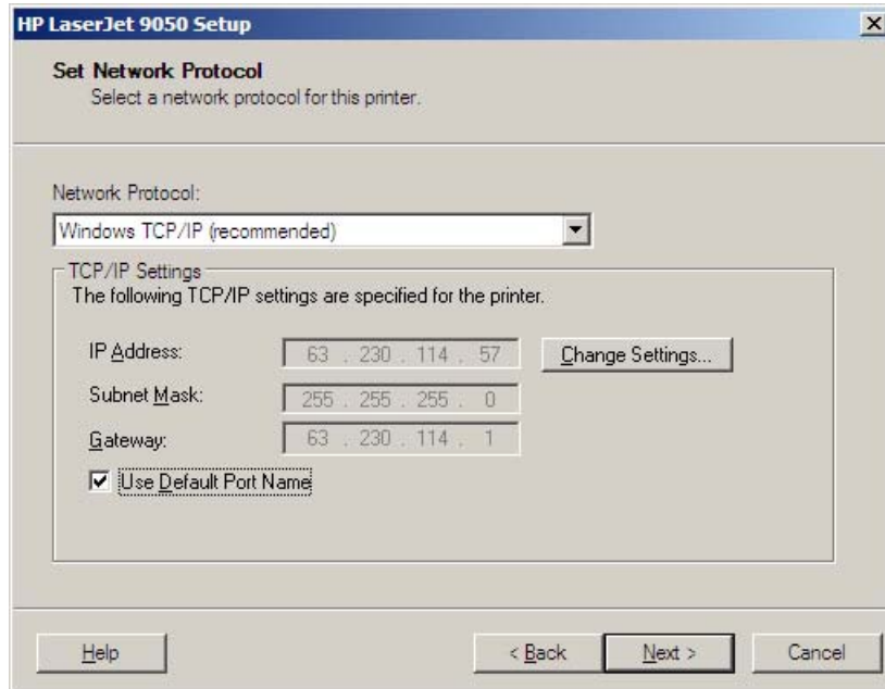
Figure 5-18 Set Network Protocol dialog box
