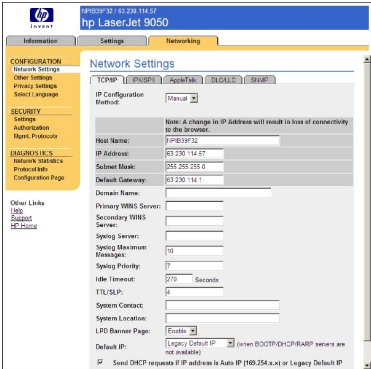
Figure 2-6 Configuration section on the Networking tab
