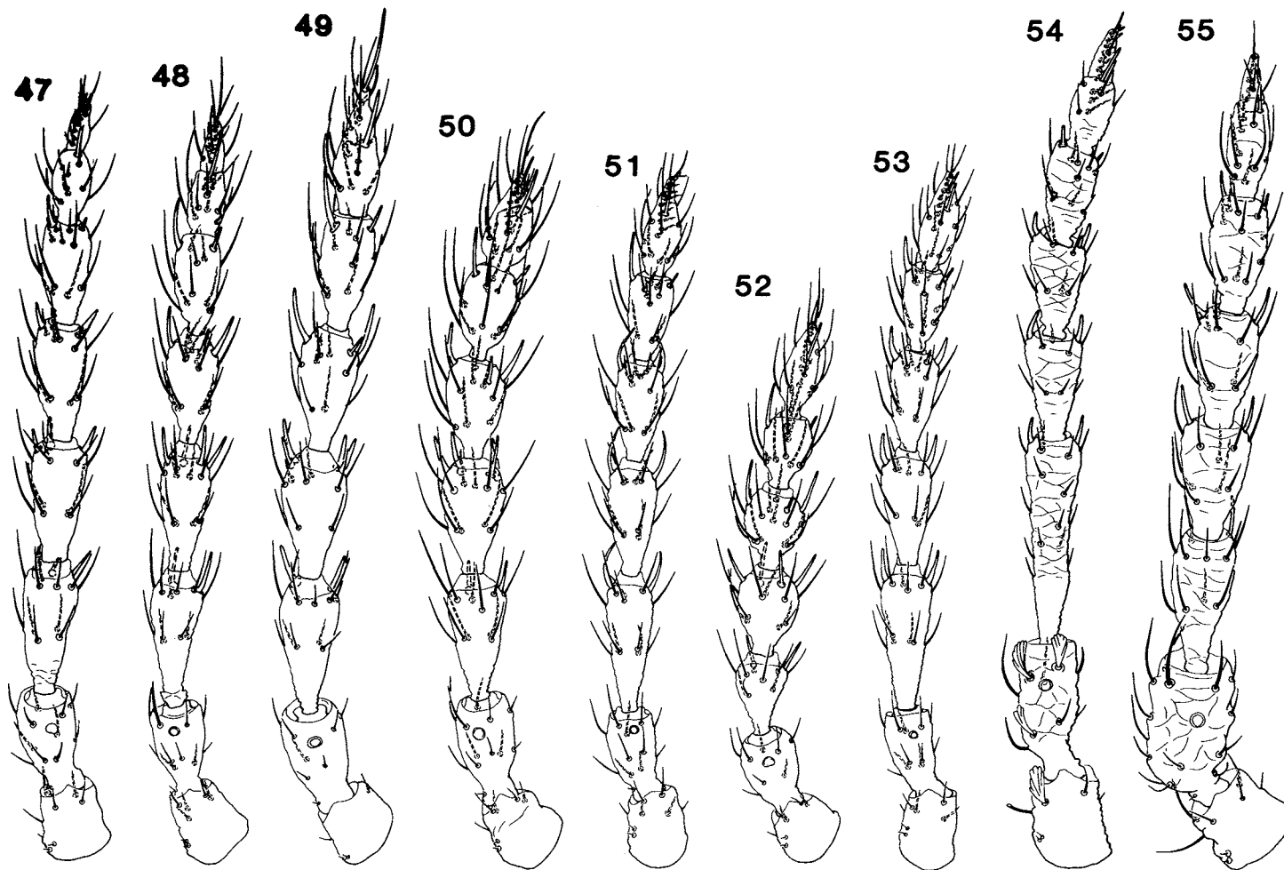
Figs 47–55 Pygothripina. 47, Cryptothrips nigripes mac.; 48, Priesneriana kabandha ; 49, Pygothrips sculpticauda ♀; 50, Ozothrips eurytis holotype; 51, O. priscus holotype; 52, O. janus holotype; 53, Heptathrips tonnoiri ; 54, Pelinothrips ornatus ; 55, Emprosthiothrips niger .
