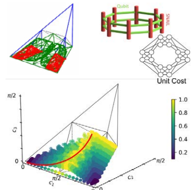
Left to Right: [smush_primitive] Candidate Basis Gates from Parallel Drive visualized in the Weyl Chamber, [corral] Corral SNAIL configuration and Qubit Coupling Topology, [coverage_set] Parallel Driven \sqrt{\text{Swap}} Decomposition Coverage Spanning Regions
