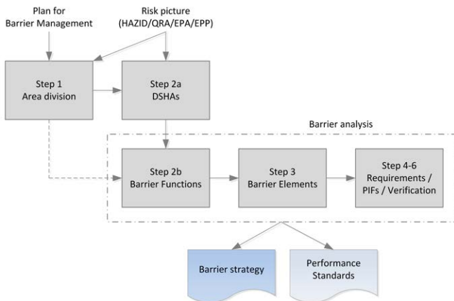
Figure 2. Typical safety barrier management process
