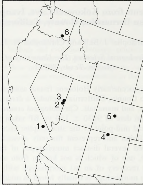
Fig. 1. Map showing location of Kokoweef Cave and other localities from which fossil mIs of Lemmings with only four closed triangles are known. 1. Kokoweef Cave and Antelope Cave; 2. Snake Creek Burial Cave; 3. Cathedral Cave; 4. SAM Cave; 5. Porcupine Cave; 6. Kennewick Roadcut.
