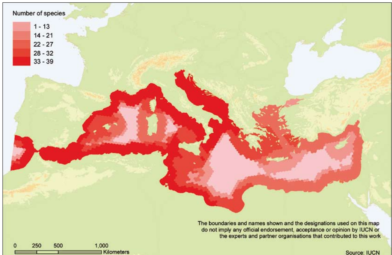
Figure 3.3 Distribution of threatened native marine fish species in the Mediterranean Sea
