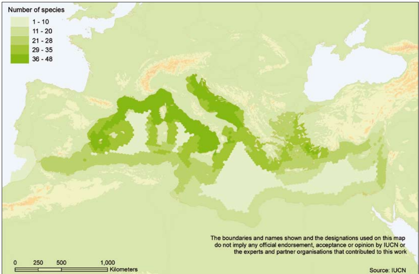
Figure 3.4 Distribution of endemic marine fish species in the Mediterranean Sea
