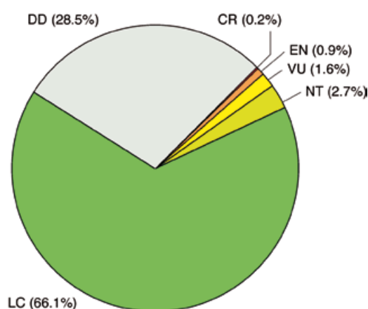
Figure 3.6. Regional Red List status of 442 native marine bony fish species in the Mediterranean Sea
