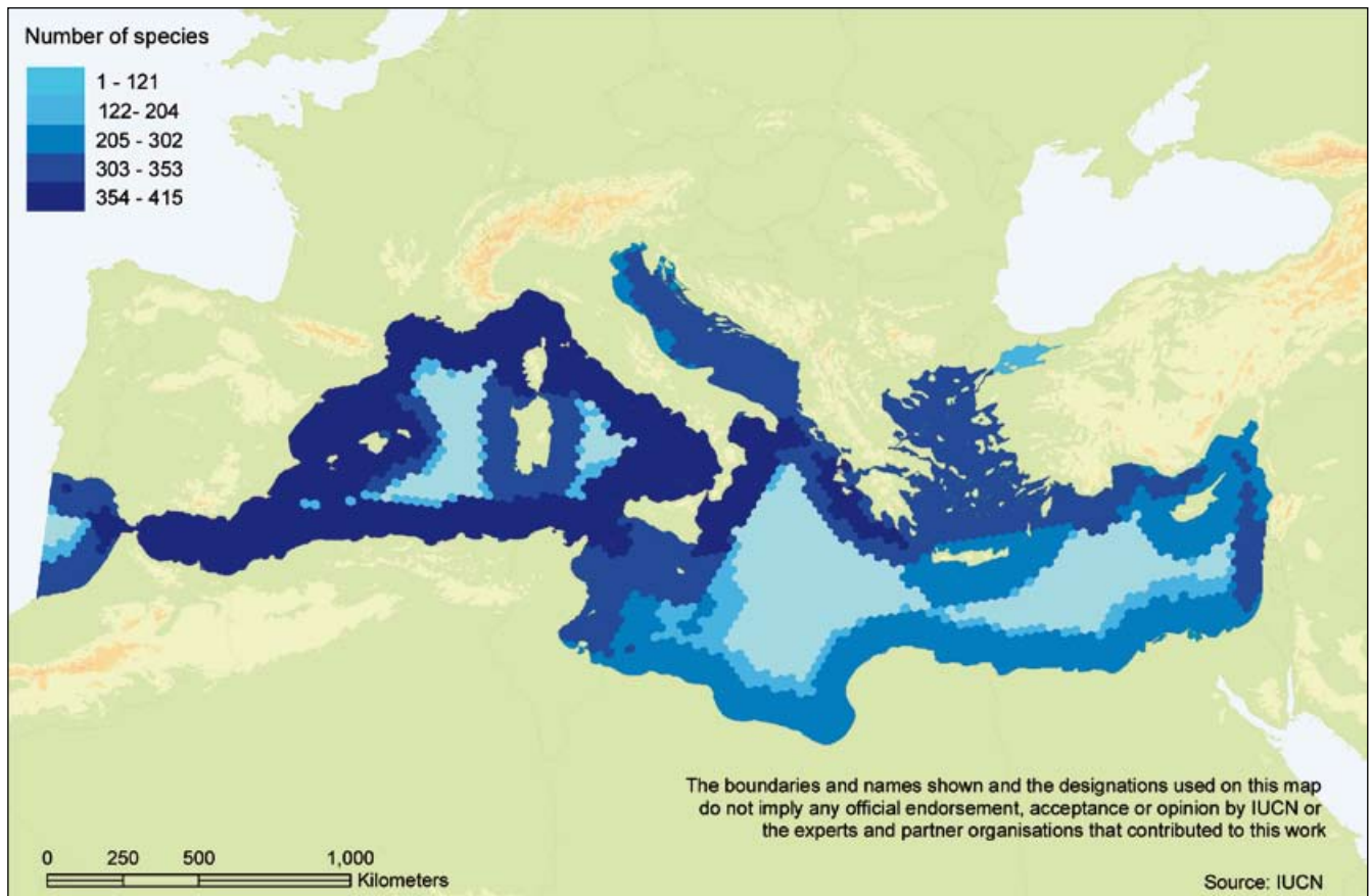
Figure 3.2 Species richness of native marine fishes in the Mediterranean Sea
