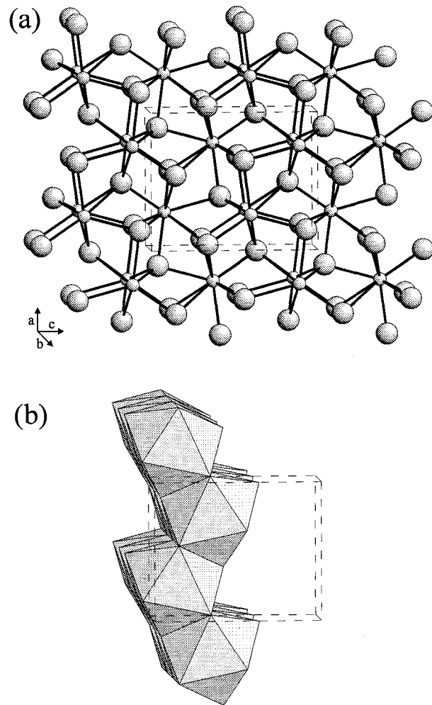
FIGURE 2. Crystal structure of \alpha - PbF_2 (Boldrini and Loopstra 1967) viewed slightly off the b axis. The unit cell is outlined by the dashed lines. (a) Ball-and-stick diagram; small balls are Pb atoms and large balls are F atoms. (b) Corrugated sheet of face-sharing Pb TCTPs; three unit cells along b are shown.
