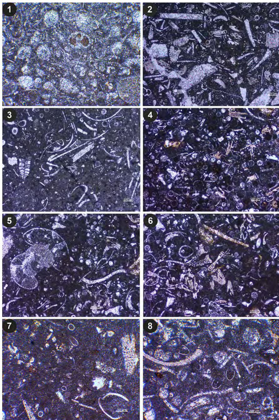
Fig. 9. Microfacies of Kóta 720: 1 – Protoglobuligerina -filamentous microfacies, sample Kóta 720-1. 2 – calpionellid- Globochaete mikrofacies, crinoids, Involutina sp., sample Kóta 720-3. 3 – calpionellid- Globochaete mikrofacies, foraminifera, bivalves, sample Kóta 720-6. 4 – radiolarian mikrofacies, crinoids, sample Kóta 720-8. 5 – calpionellid-radiolarian mikrofacies, juvenile ammonites, sample Kóta 720-12. 6 – calpionellid-radiolarian mikrofacies, crinoids, Spirulina sp., sample Kóta 720-12. 7 – bioclastic limestone with Calpionellopsis oblonga Cadisch and crinoids, sample Kóta 720-8.5. 8 – bioclastic limestone with Calpionellites sp., sample Kóta 720-15. Light microscope Leica DM 2500 with Axiacam ERc 5s digital camera.
