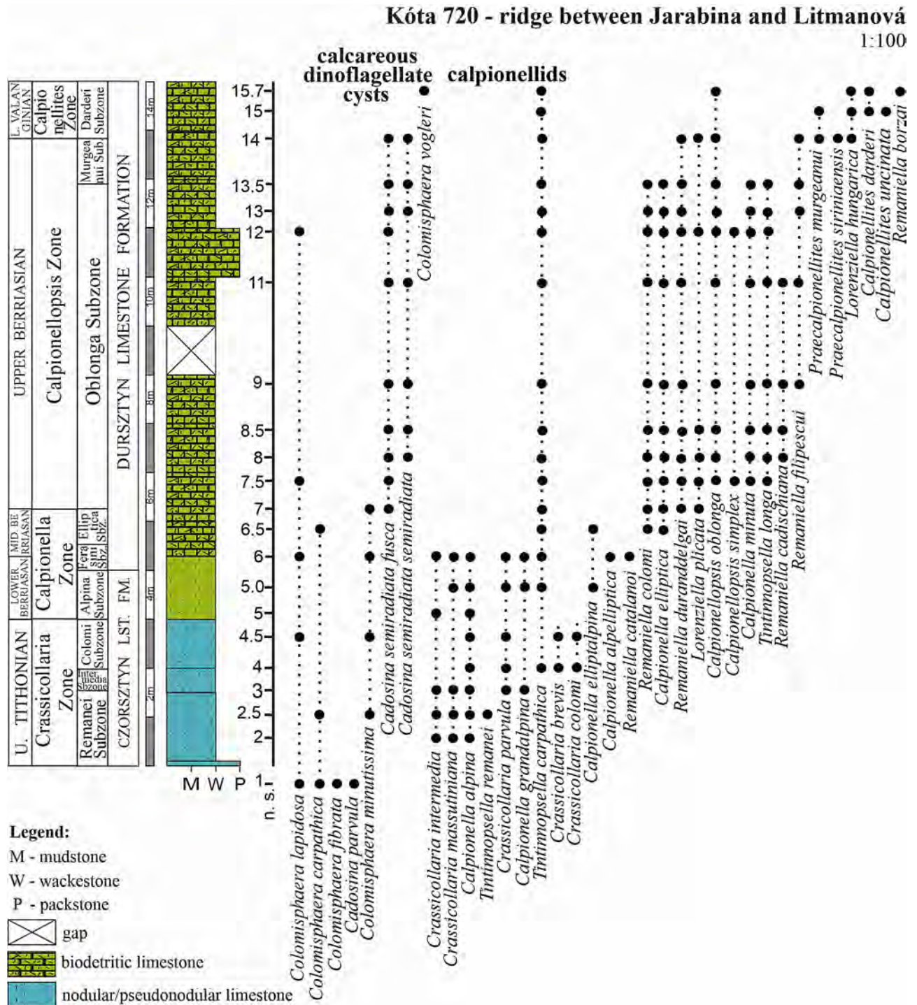
Fig. 8. Distribution of calcareous dinoflagellates and calpionellids in Kóta 720 section with calpionellid and dinoflagellate cysts biozonation.
