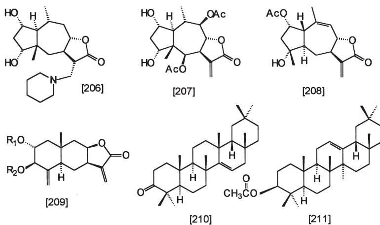
Fig. 2.63 Compounds 206, an alkaloid, and 207–209, sesquiterpenes from Gaillardia pulchella . Compounds 210 and 211, triterpenes from Dudleya
