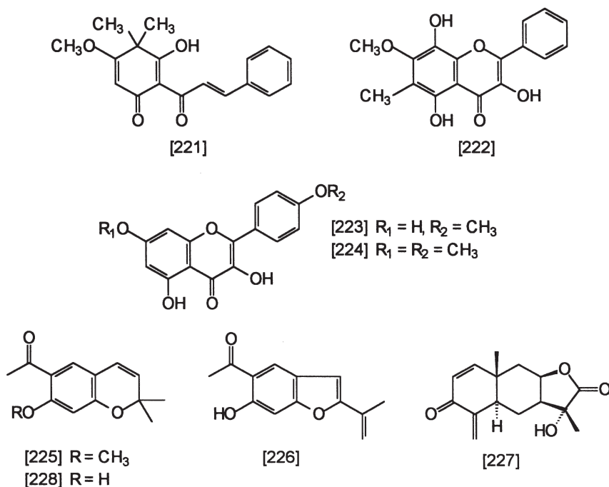
Fig. 2.69 Compounds 221–224, flavonoids of Pentagramma ( Pityrogramma ) triangularis . Compounds 225–228 from Encelia farinosa
