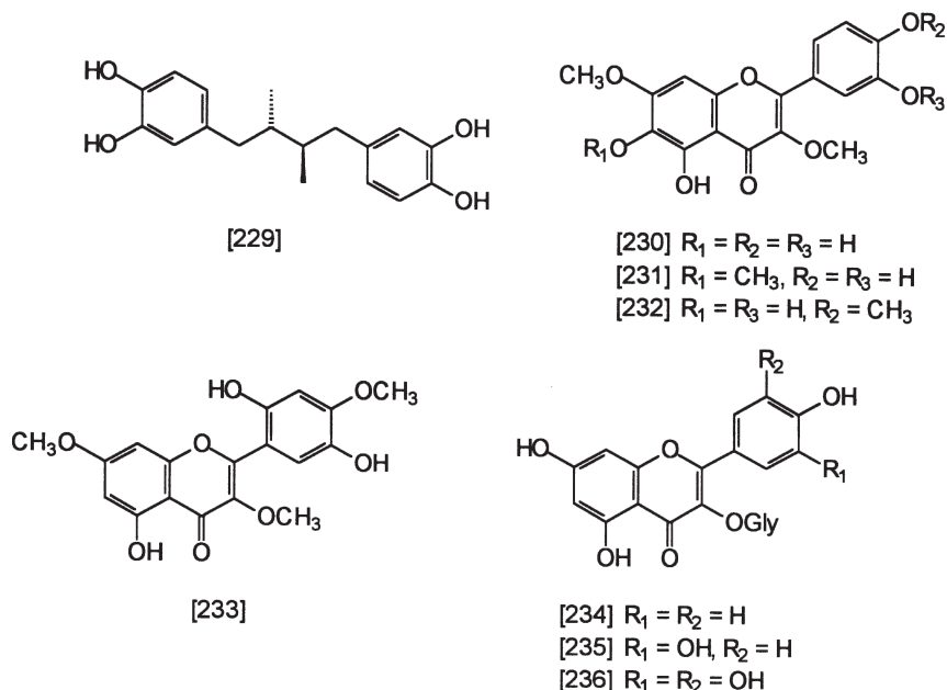
Fig. 2.71 Compound 229 from Larrea tridentata . Compounds 230–233, flavonoids from Chryso-splenium glechomaeifolium . Compounds 234–236, flavonoids from Quercus rubra
