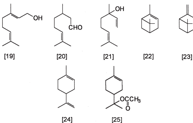
Fig. 2.5 Compounds 19–25 from Chamelaucium uncinatum , the Geraldton waxflower
