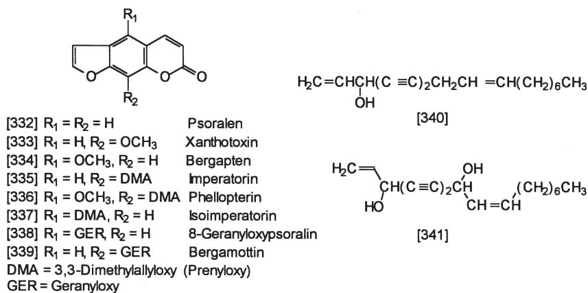
Fig. 4.10 Compounds 332–341, coumarins and acetylene derivatives from Glehnia
