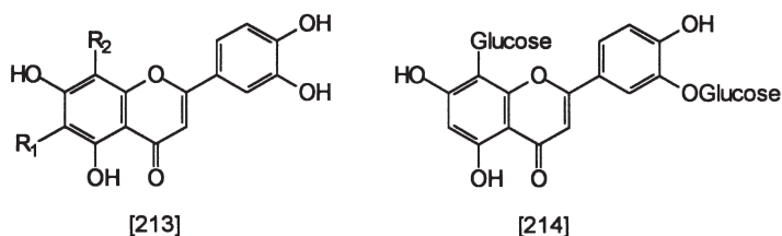
Fig. 2.66 Compounds 213 and 214, key flavonoids from Lupinus sericeus study
