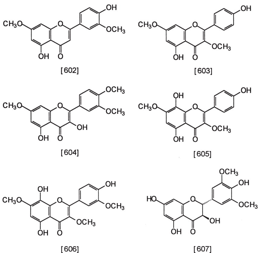
Fig. 7.4 Compounds 602–607, flavonoids from Larrea tridentata
