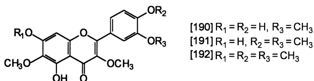
Fig. 2.58 Compounds 190–192, flavonoids from Brickellia cylindrica
