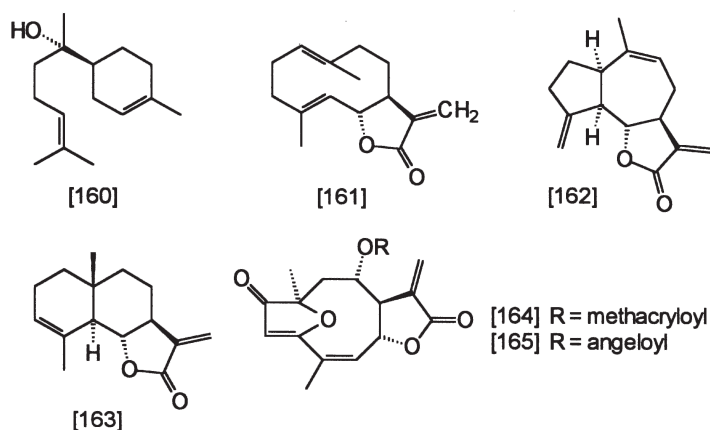
Fig. 2.42 Compounds 160–165, sesquiterpenes from Vanillosmopsis erythropappa
