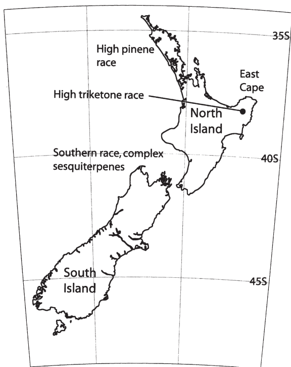
Fig. 2.11 Map of New Zealand showing general locations of the three chemotypes of Leptospermum scoparium
