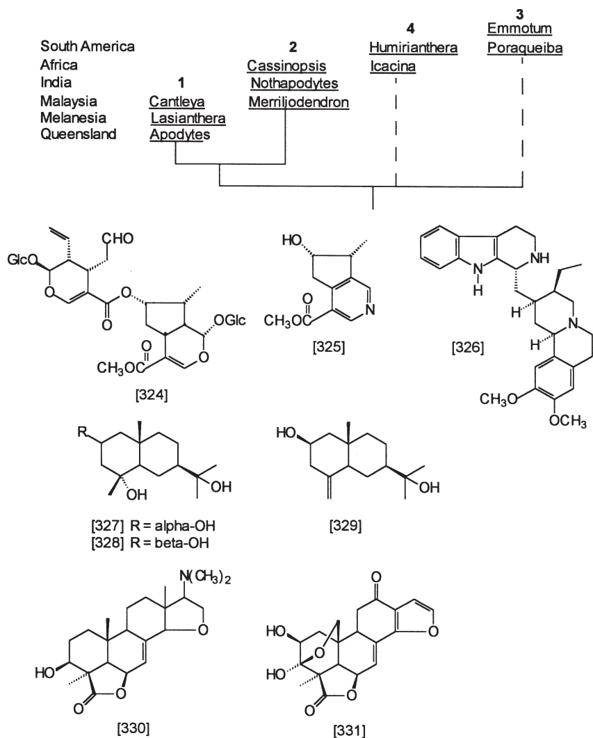
Fig. 4.8 Compounds 324–331, terpenoids and alkaloids from some Icacinaceae
