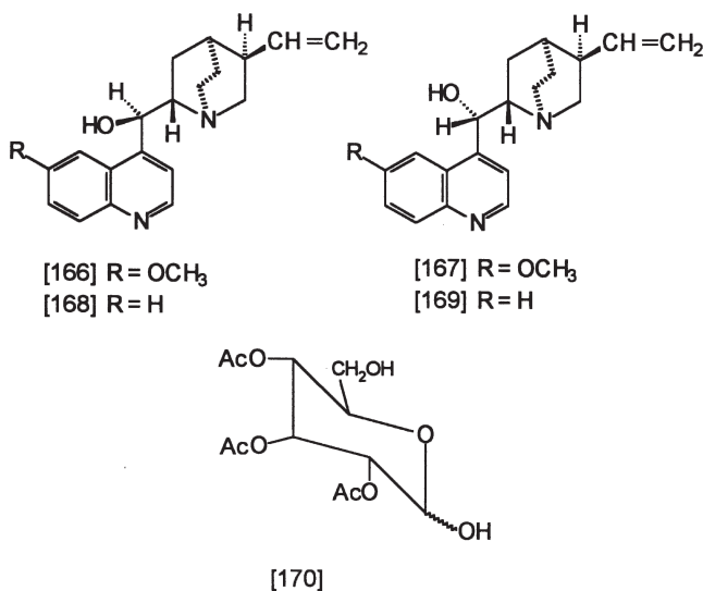
Fig. 2.43 Compounds 166–169, quinine relatives from Cinchona . Compound 170, a generalized sugar ester from Lycopersicon pennellii
