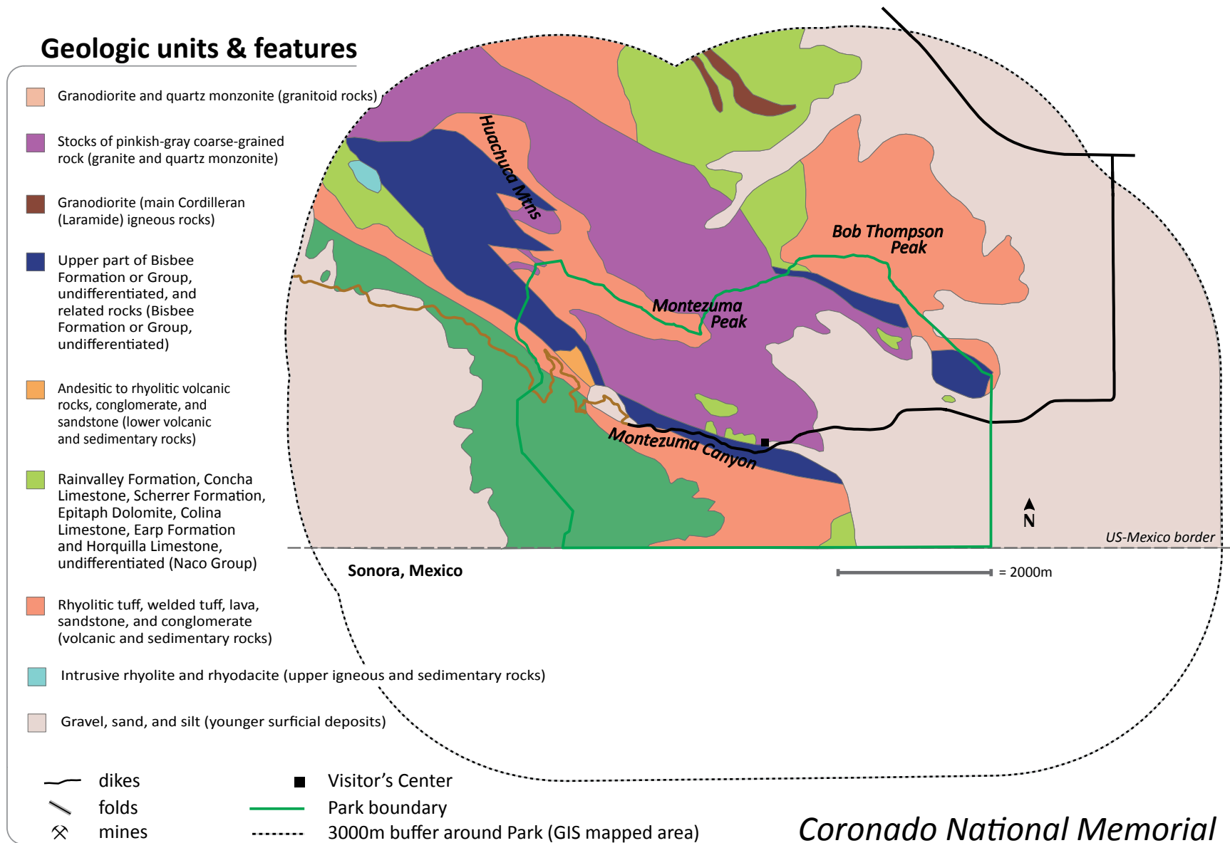
Figure 4.2. Surface geology at Coronado NMem.
