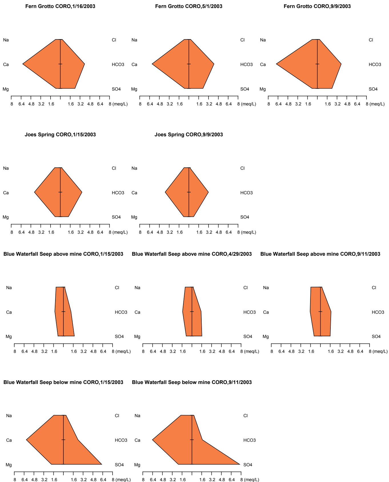
Figure B.7. Stiff diagrams of major ions in Coronado NM water quality samples.
