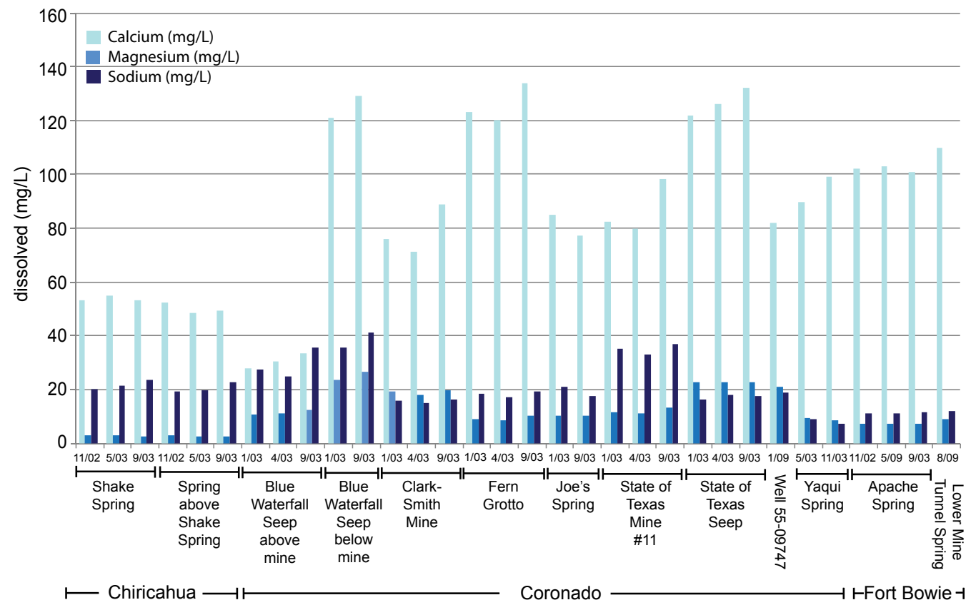
Figure B.15. Calcium, magnesium, and sodium results from Chiricahua NM, Coronado NMem, and Fort Bowie NHS water quality samples.
