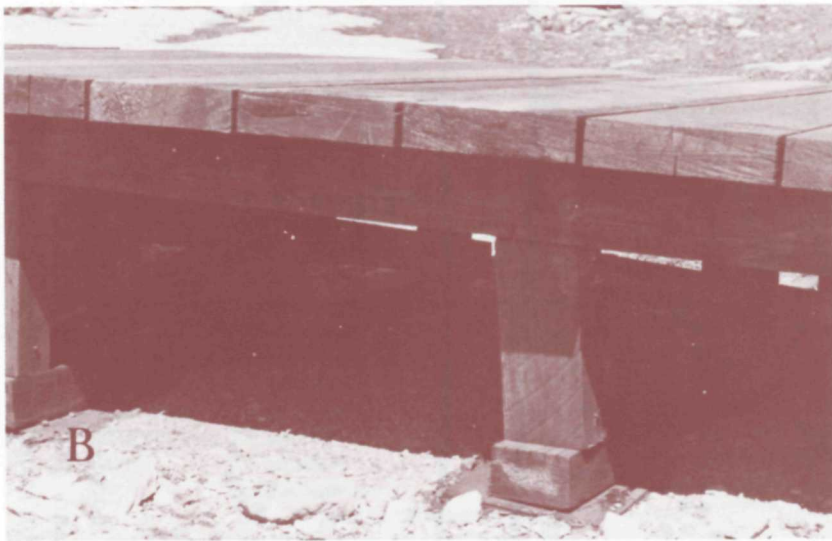
FIGURE 2. (A) Study area along wooden walkway, Logan Pass, Glacier National Park, showing: a. affected area south of walkway, b. affected area north of walkway, c. unaffected control area. (B) Construction details of wooden walkway showing dark colored, heavily treated lumber.
