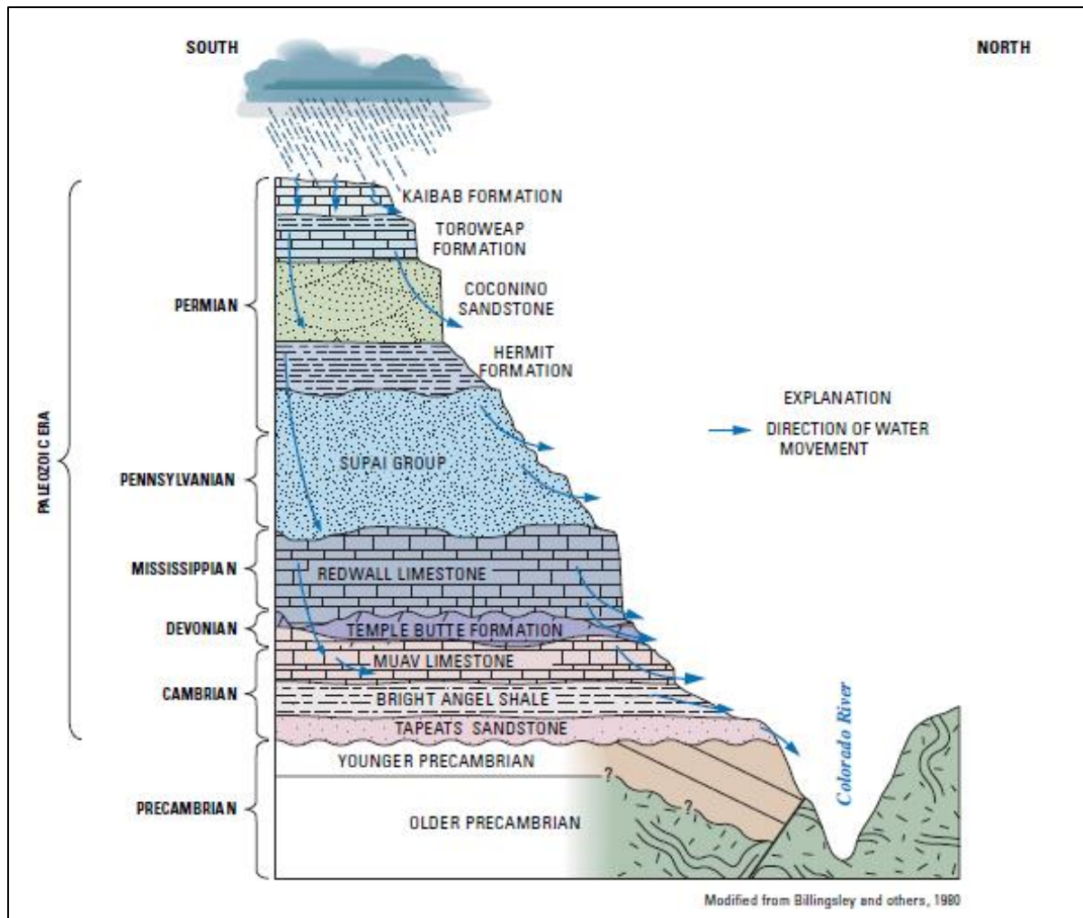
Figure 6. Stratigraphic section depicting water flow through the geologic strata of the Grand Canyon's South Rim (modified from Billingsley et al. 1980).
