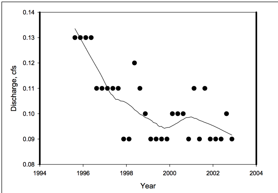
Figure 60. Median quarterly discharge at Pumphouse Creek with a locally weighted scatterplot smooth line (From Rihs et al. 2004).
