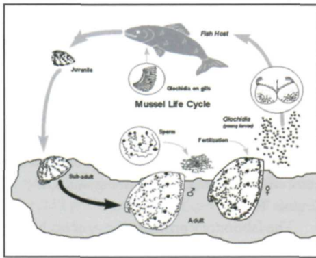
Figure 1. The life cycle of freshwater mussels, showing their development from parasitic larvae, called glochidia, on fish gills (often with particular mussel species dependent on specific fish hosts), to sedentary, filter-feeding adults.
