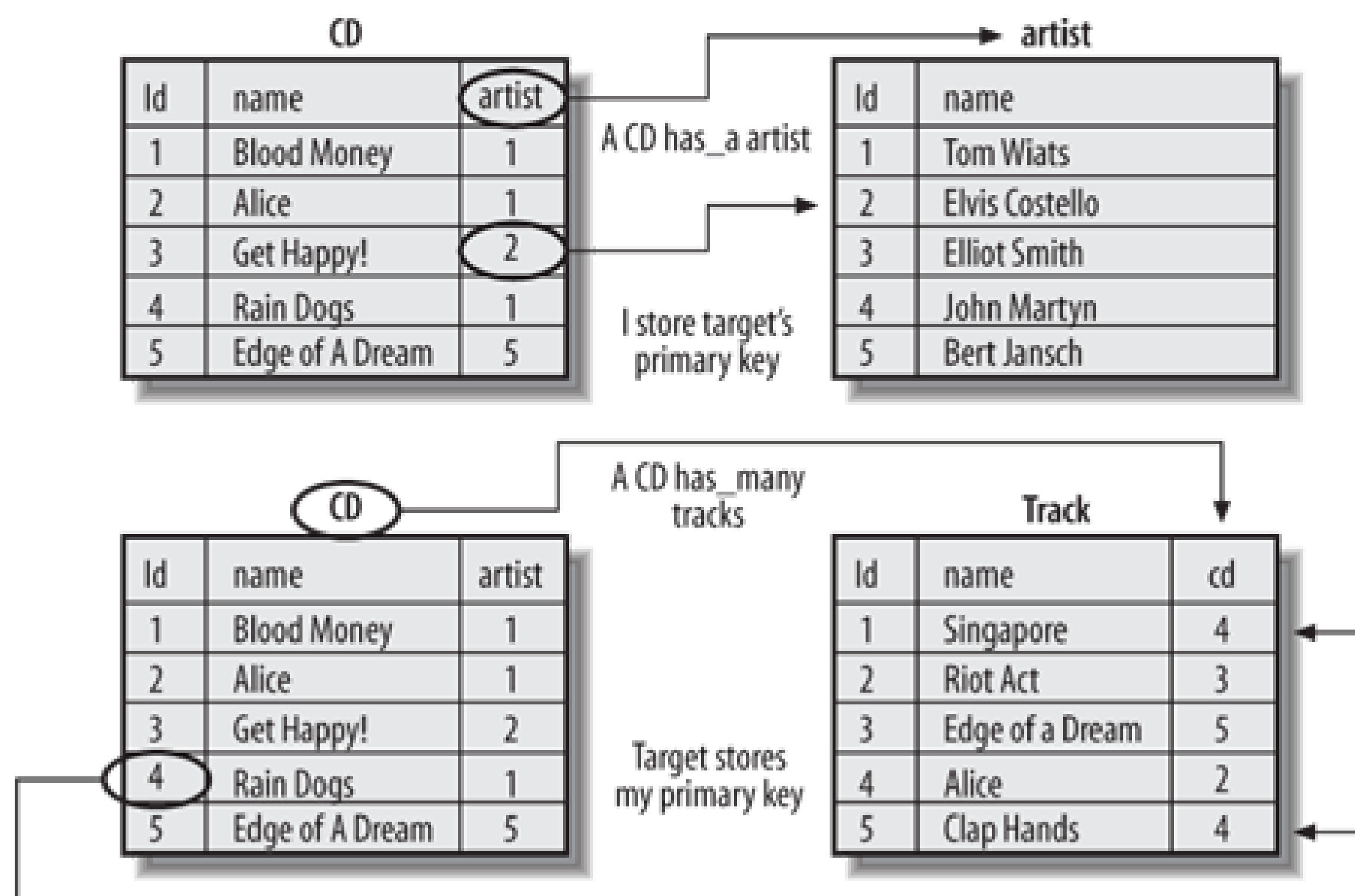
Figure 4-1. has_a versus has_many
