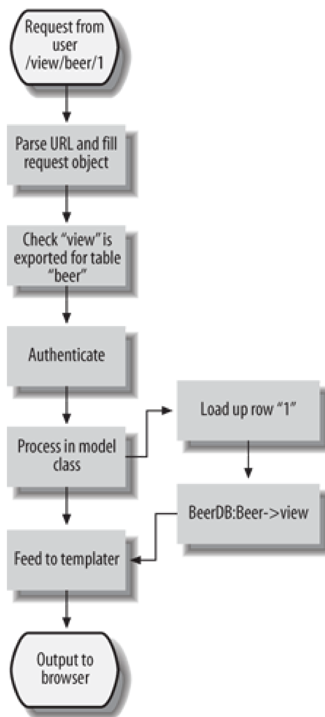
Figure 4-3. The Maypole work flow
