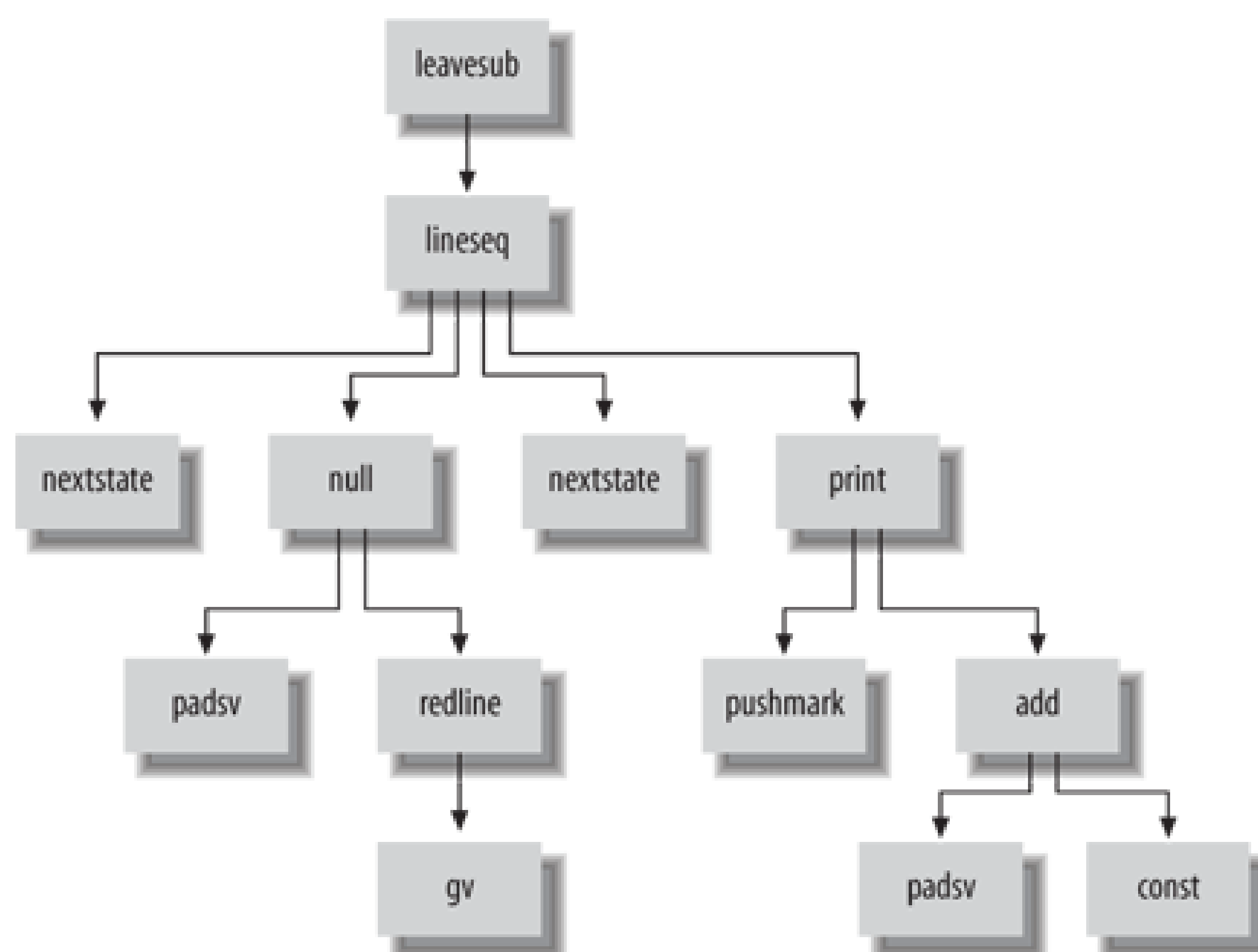
Figure 1-5. Bytecode tree
