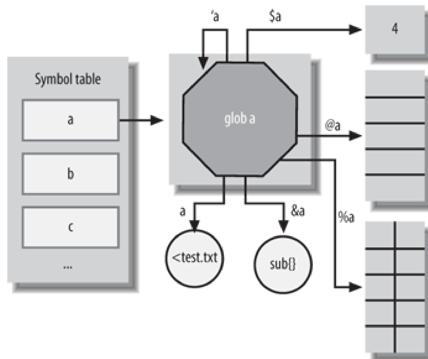
Figure 1-2. Consulting the symbol table, take 2
