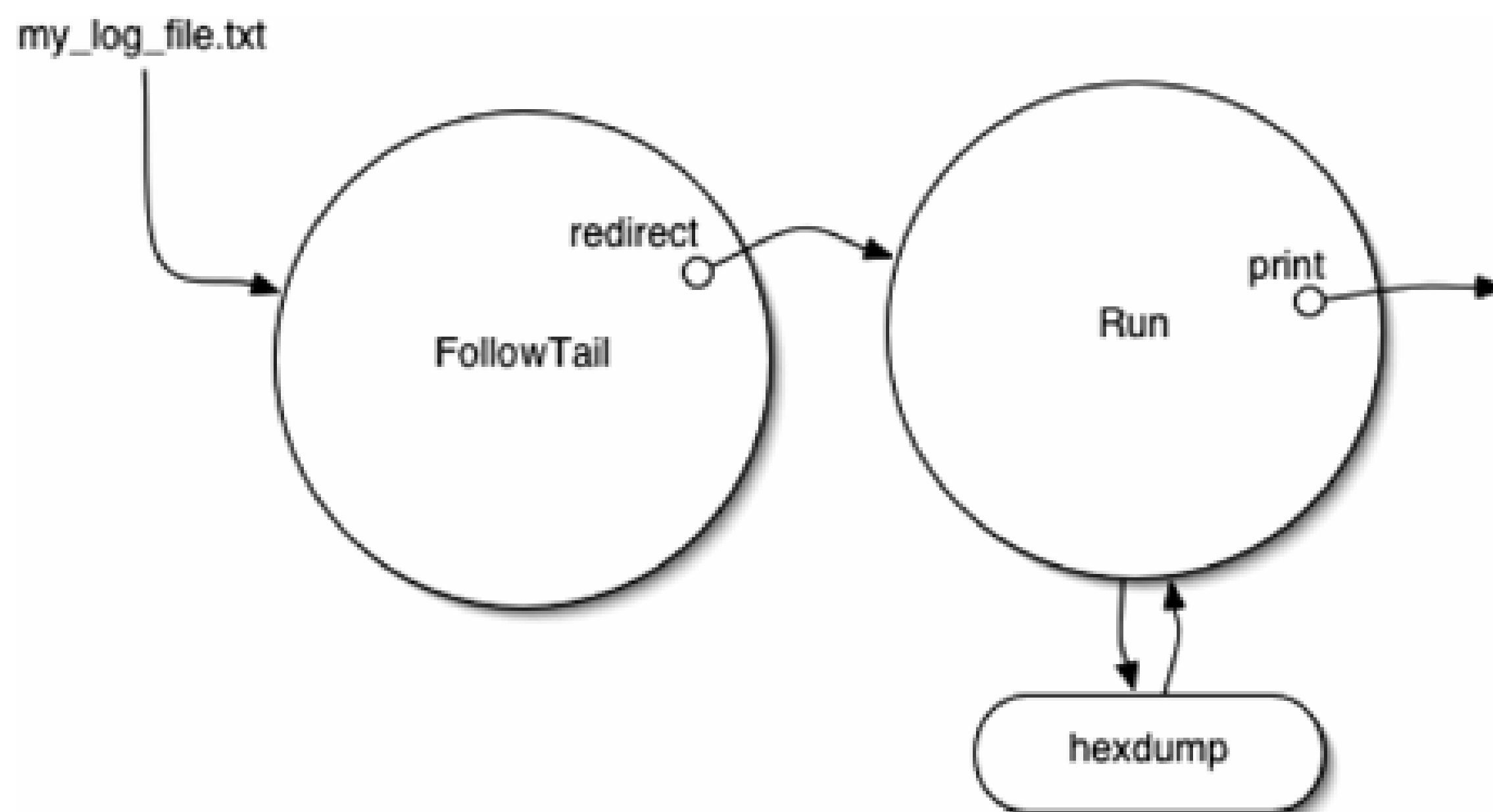
Figure 7-1. Filtered log tailing
