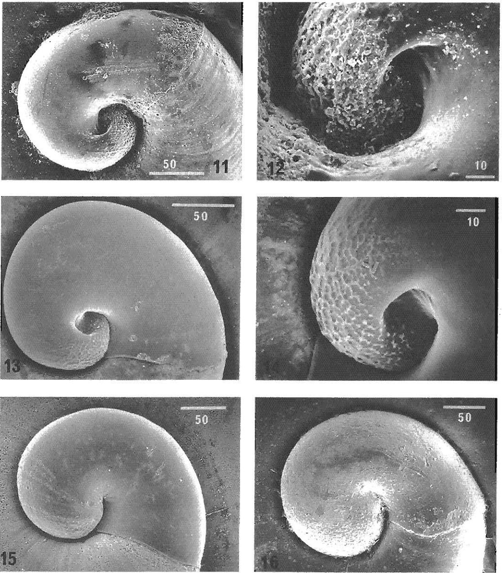
Figures 11-16. Hyalogyrina amphorae Warén, Carozza & Rocchini, sp. n. protoconch morphology and deposition of calcium carbonate. 11-12. Paratype. 13-14. Another paratype with centre of protoconch starting to get covered. 15. Protoconch with centre completely covered. Akritogyra conspicua (Monterosato), protoconch. Scale lines in \mu\text{m} .
