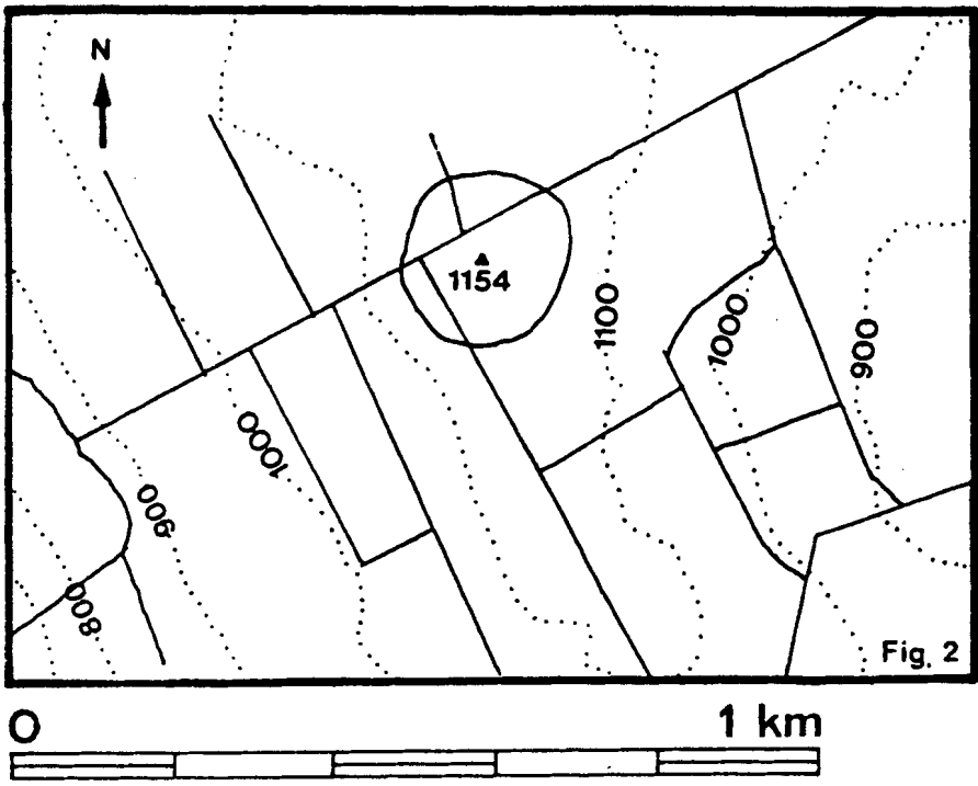
FIG.2: Sketch plan of Clomantagh Hillfort. Trig. station is situated on cairn. (Based on Ordnance Survey).
