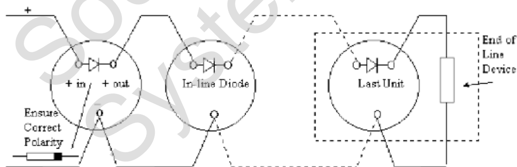
Fig. 1.2 Detector Wiring diagram
