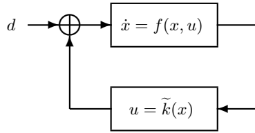
Fig. 9. Different feedback ISS-stabilizes
