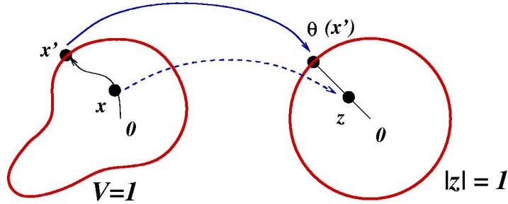
Fig. 28. Making level sets into spheres
