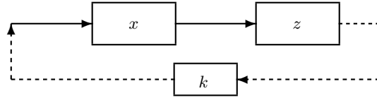
Fig. 13. Adding a feedback to the cascade
