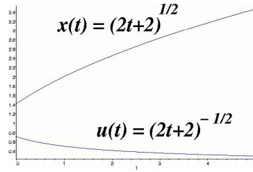
Fig. 5. Diverging state for converging input, for example
