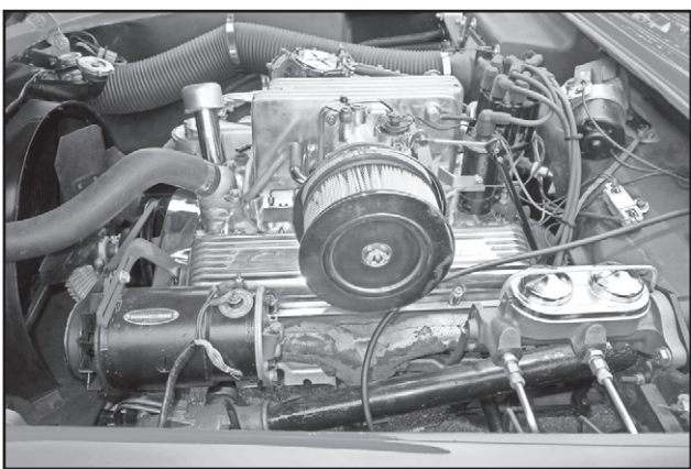
The 1957 Corvette 283 cubic inches, 250 HP engine with fuel injection and air cleaner showing also upgraded brake dual master cylinder
