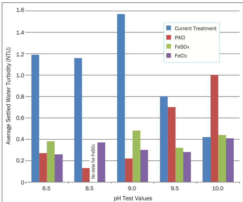
Figure 11. Effect of pH on coagulant performance. Notes: Raw turbidity, 2.7-10 NTU Raw alkalinity, 68-81 mg/L as CaCO 3 Water temperature, 14°C-29°C
