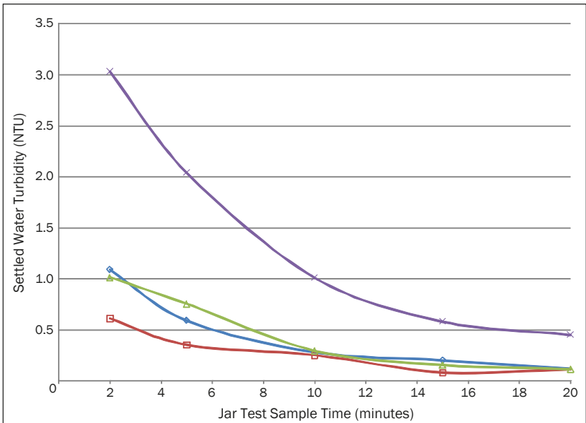
Figure 12. Effect of CO 2 on pH adjustment and PACl performance. Notes: Raw turbidity, 2.8 NTU PACl dosage, 0.073 mmole Al (35 mg/L PACl product)
