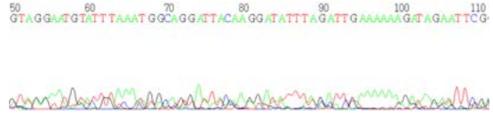
FIGURE 10. Part of the sequence of the gene matK of the species Prostecchia grammatoglossa 2011 (Quintanilla et al. 2010).
