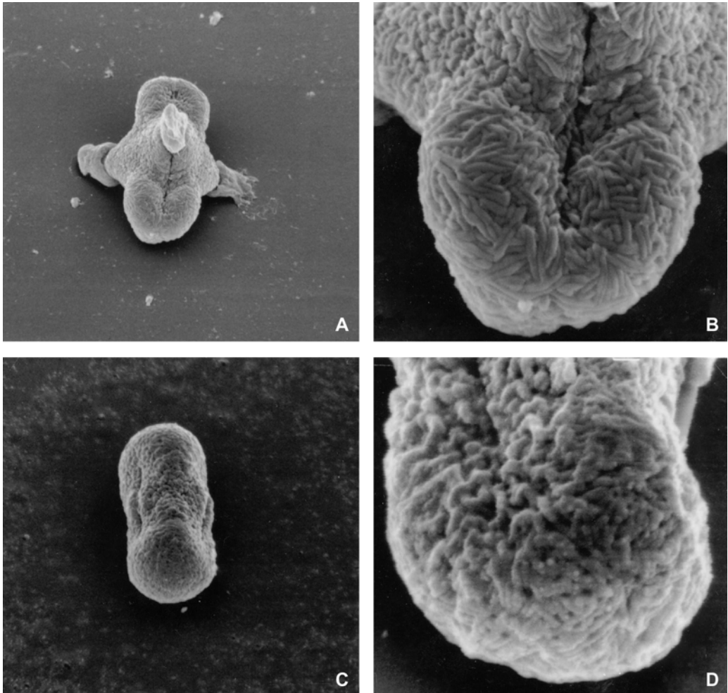
Fig. 5: SEM pictures of pollen grains in Zosima species. A, B) three-colporate pollen grain with striate-rugulate surface in Zosima gilliana ; C, D) three-colporate pollen grain with cerebriform surface in Z. absinthifolia .
