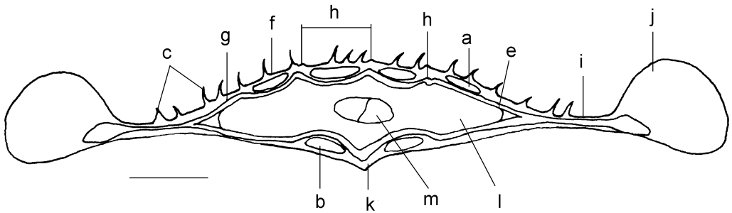
Fig. 3: Transverse section of a mericarp of Z. radians (a - dorsal vitta, b - commissural vitta, c - hairs, d - vallecular region (the distance between two ribs), e - endocarp, f - exocarp, g - mesocarp, h - dorsal vascular bundle, i - mericarp wing neck, j - mericarp wing margin, k - carpophore, l - endosperm, m - cotyledon). Scale 1 mm.
