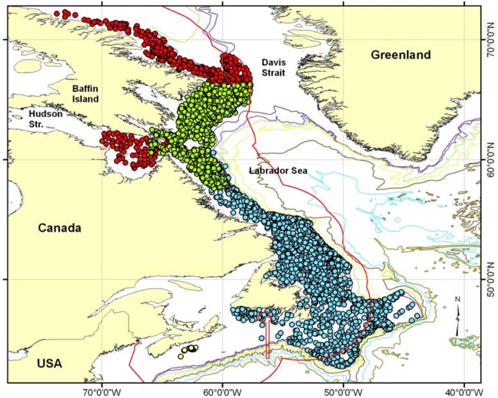
Figure 8.2.2.2. Map of the areas covered in surveys by the DFO Newfoundland Region (blue), the DFO Central and Arctic Region (red) and by the NSRF/DFO joint survey (green), and used in this report to assess sponge distribution. Similar data were not available for mapping from DFO Maritimes Region but the locations of the Russian Hats are indicated in yellow. The red line indicates the Canadian EEZ. Depth contours beginning at 1000 m and at 500 m intervals to 4000 m are displayed.
