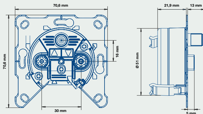
Socket body
